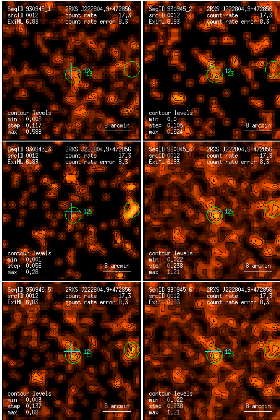
Figure 12: RASS 930945: detection 0012: band rate images, Gaussian filter: (1) PSPC channels 11 – 41, (2) 52 – 90, (3) 91 – 201, (4) 11 – 235, (5) 52 – 201, (6) 11 – 201. Broad band rates in counts/ks. Band rate contour levels in counts/ks/arcmin 2 .
