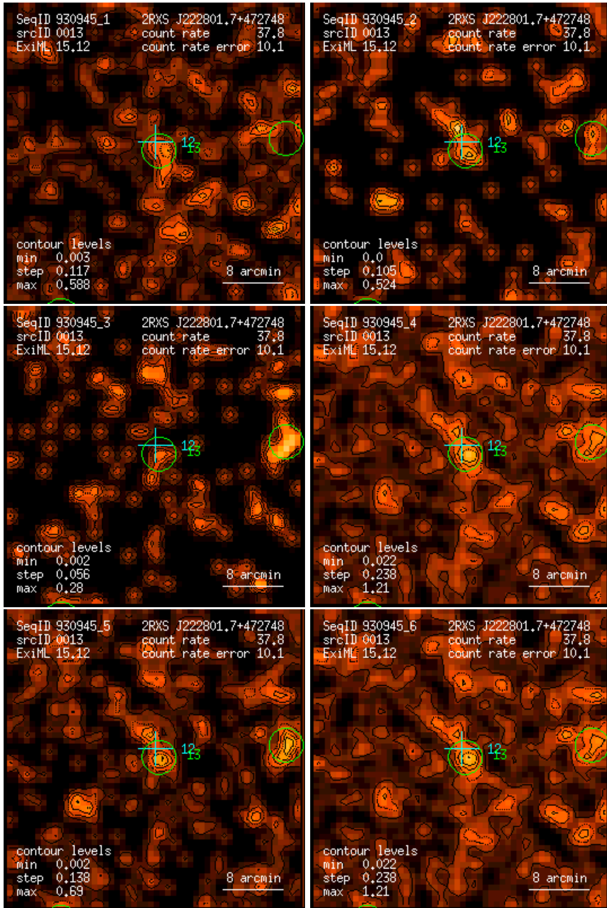
Figure 13: RASS 930945: detection 0013: band rate images, Gaussian filter: (1) PSPC channels 11 – 41, (2) 52 – 90, (3) 91 – 201, (4) 11 – 235, (5) 52 – 201, (6) 11 – 201. Broad band rates in counts/ks. Band rate contour levels in counts/ks/arcmin 2 .
