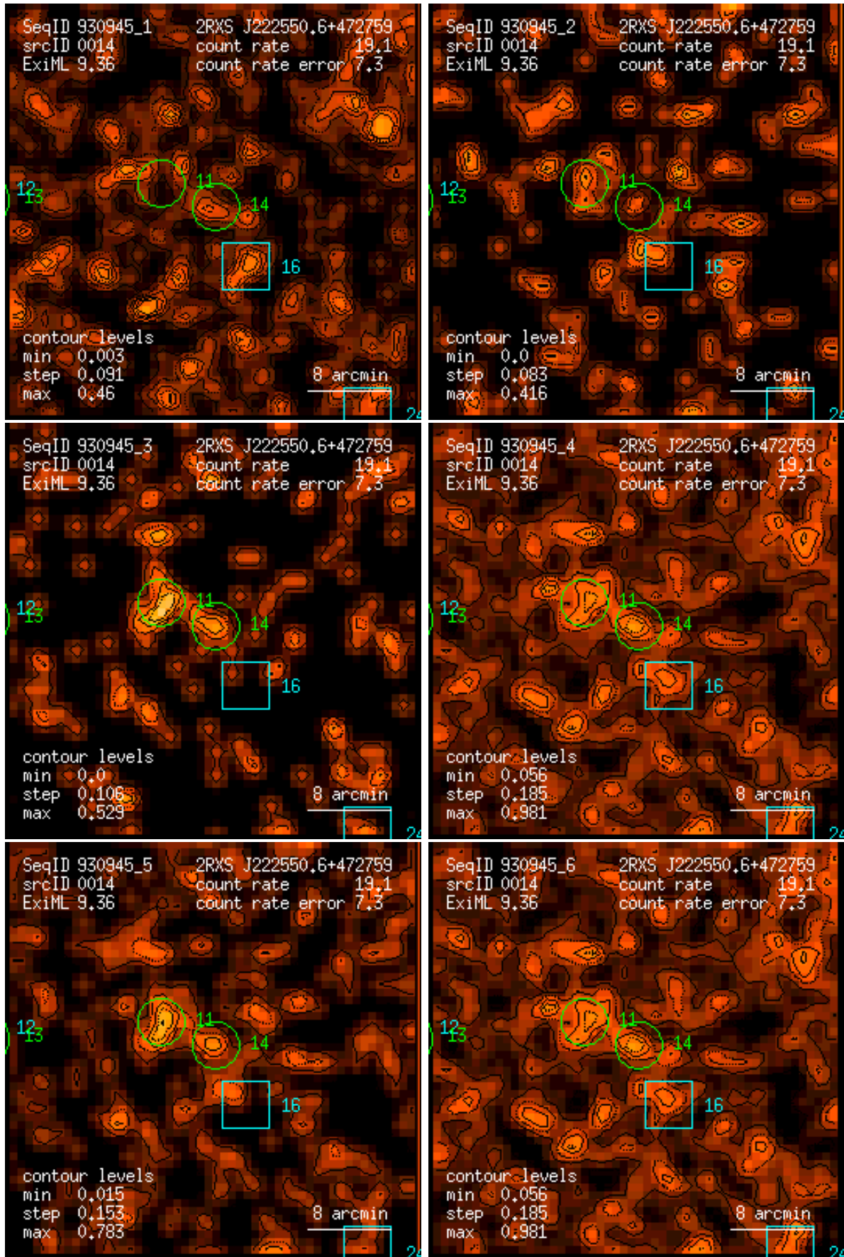
Figure 14: RASS 930945: detection 0014: band rate images, Gaussian filter: (1) PSPC channels 11 – 41, (2) 52 – 90, (3) 91 – 201, (4) 11 – 235, (5) 52 – 201, (6) 11 – 201. Broad band rates in counts/ks. Band rate contour levels in counts/ks/arcmin 2 .
