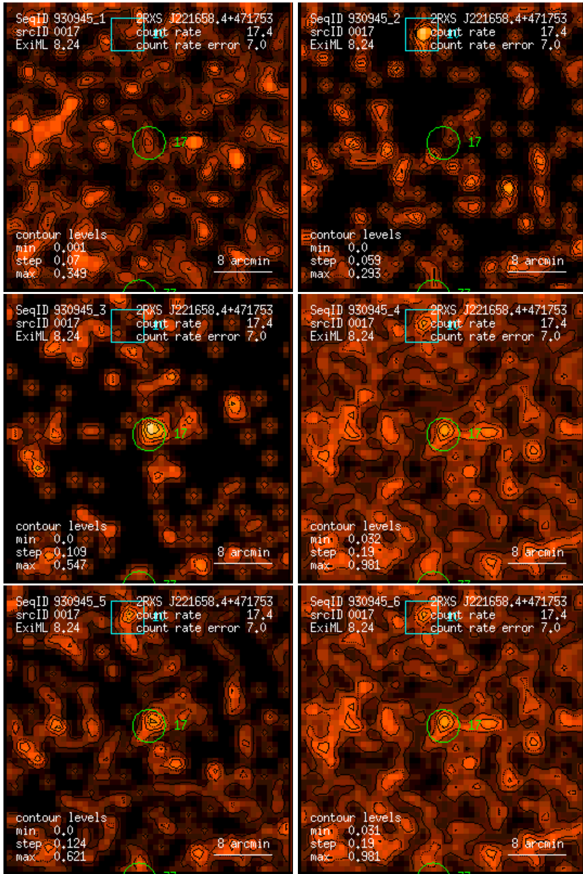
Figure 17: RASS 930945: detection 0017: band rate images, Gaussian filter: (1) PSPC channels 11 – 41, (2) 52 – 90, (3) 91 – 201, (4) 11 – 235, (5) 52 – 201, (6) 11 – 201. Broad band rates in counts/ks. Band rate contour levels in counts/ks/arcmin 2 .
