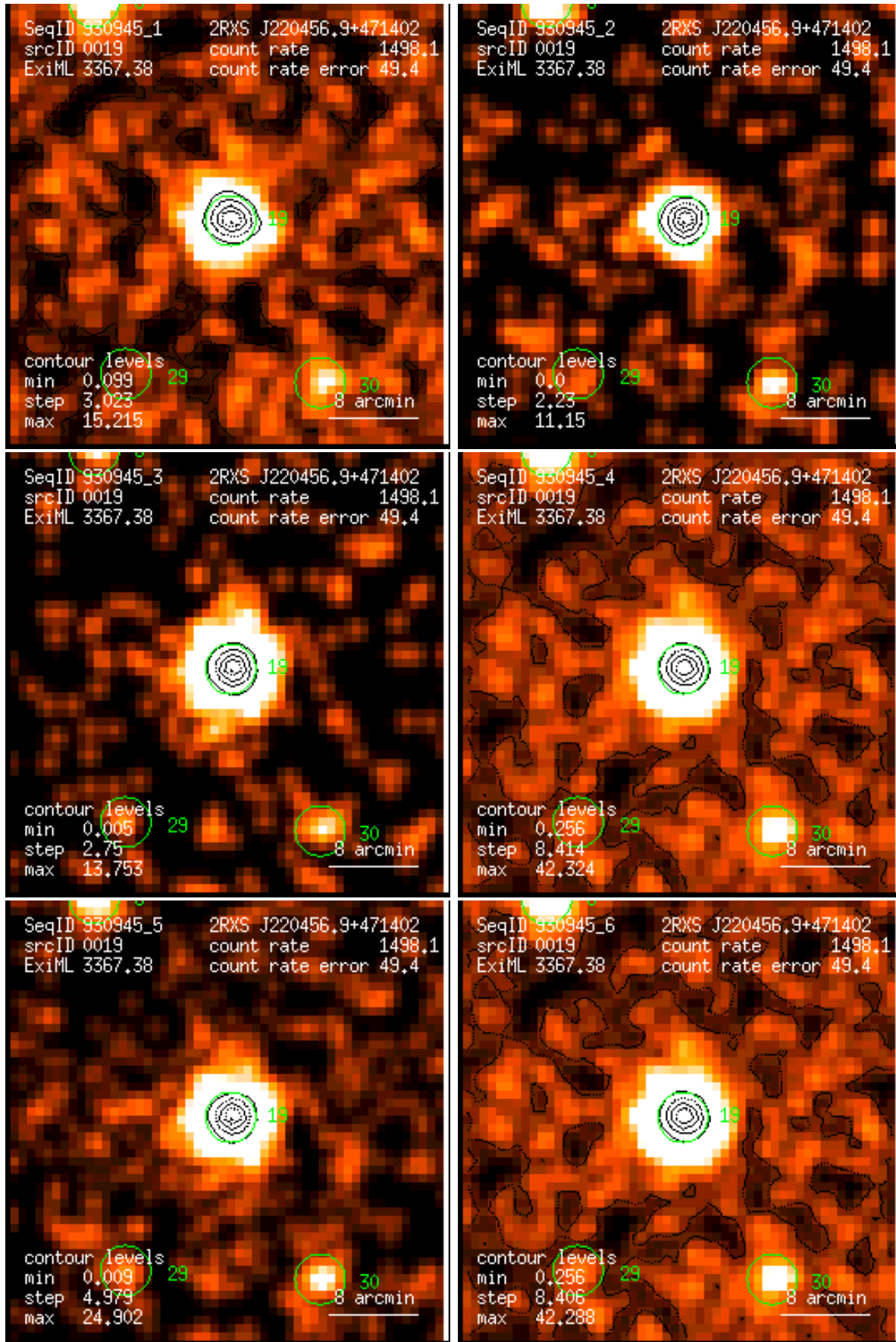
Figure 19: RASS 930945: detection 0019: band rate images, Gaussian filter: (1) PSPC channels 11 – 41, (2) 52 – 90, (3) 91 – 201, (4) 11 – 235, (5) 52 – 201, (6) 11 – 201. Broad band rates in counts/ks. Band rate contour levels in counts/ks/arcmin 2 .
