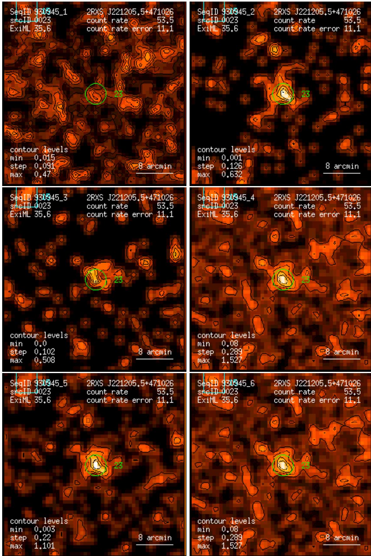
Figure 23: RASS 930945: detection 0023: band rate images, Gaussian filter: (1) PSPC channels 11 – 41, (2) 52 – 90, (3) 91 – 201, (4) 11 – 235, (5) 52 – 201, (6) 11 – 201. Broad band rates in counts/ks. Band rate contour levels in counts/ks/arcmin 2 .
