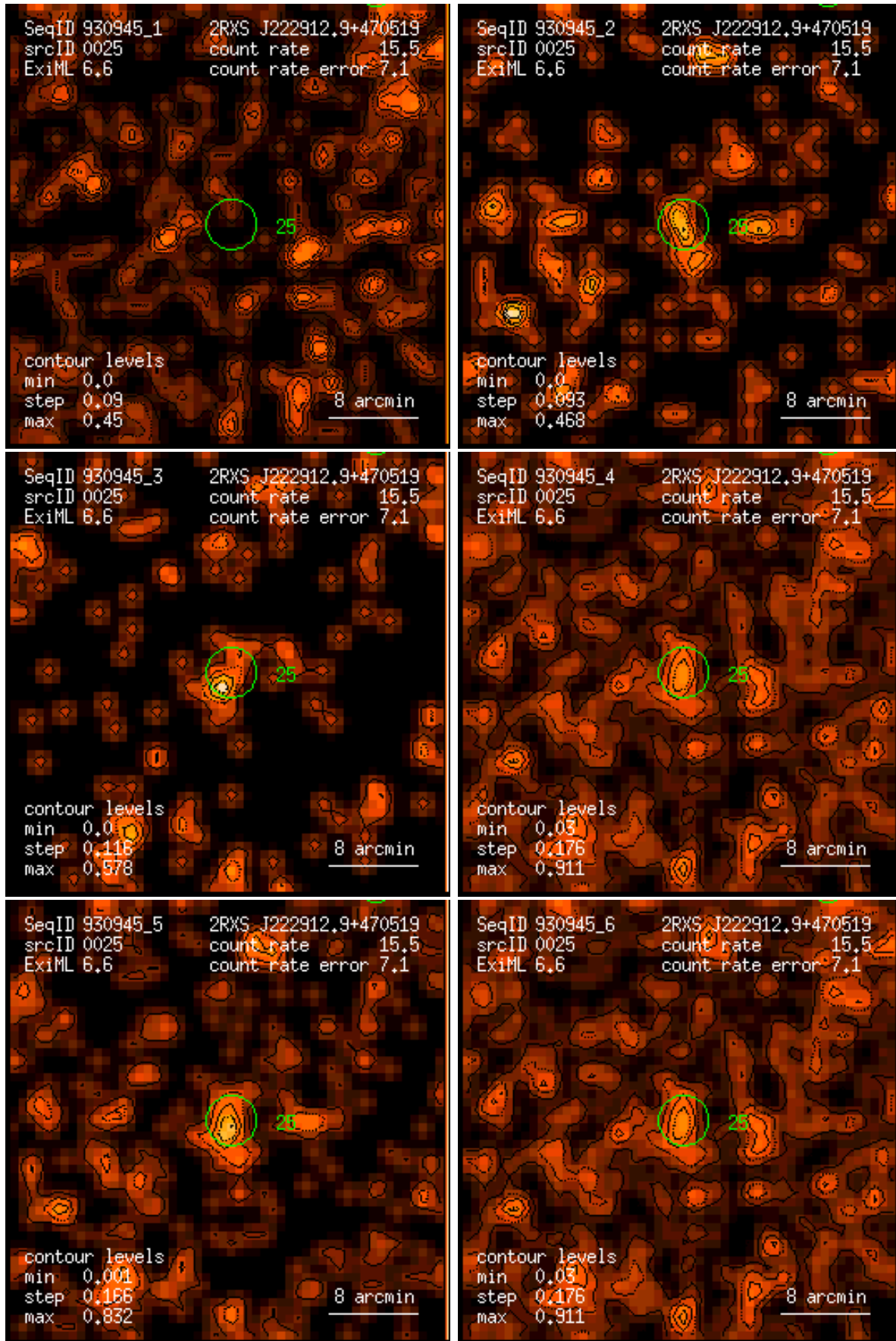
Figure 25: RASS 930945: detection 0025: band rate images, Gaussian filter: (1) PSPC channels 11 – 41, (2) 52 – 90, (3) 91 – 201, (4) 11 – 235, (5) 52 – 201, (6) 11 – 201. Broad band rates in counts/ks. Band rate contour levels in counts/ks/arcmin 2 .
