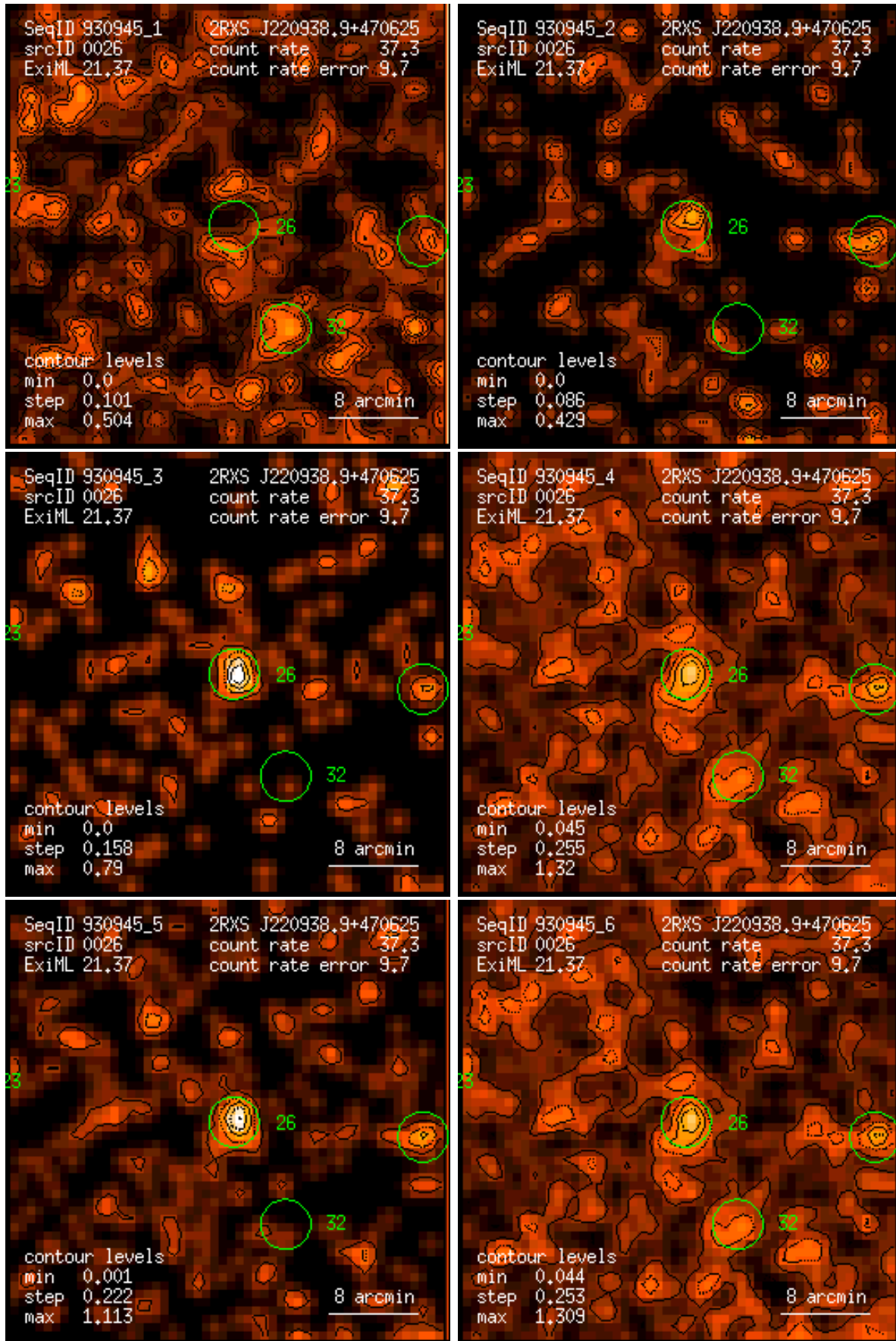
Figure 26: RASS 930945: detection 0026: band rate images, Gaussian filter: (1) PSPC channels 11 – 41, (2) 52 – 90, (3) 91 – 201, (4) 11 – 235, (5) 52 – 201, (6) 11 – 201. Broad band rates in counts/ks. Band rate contour levels in counts/ks/arcmin 2 .
