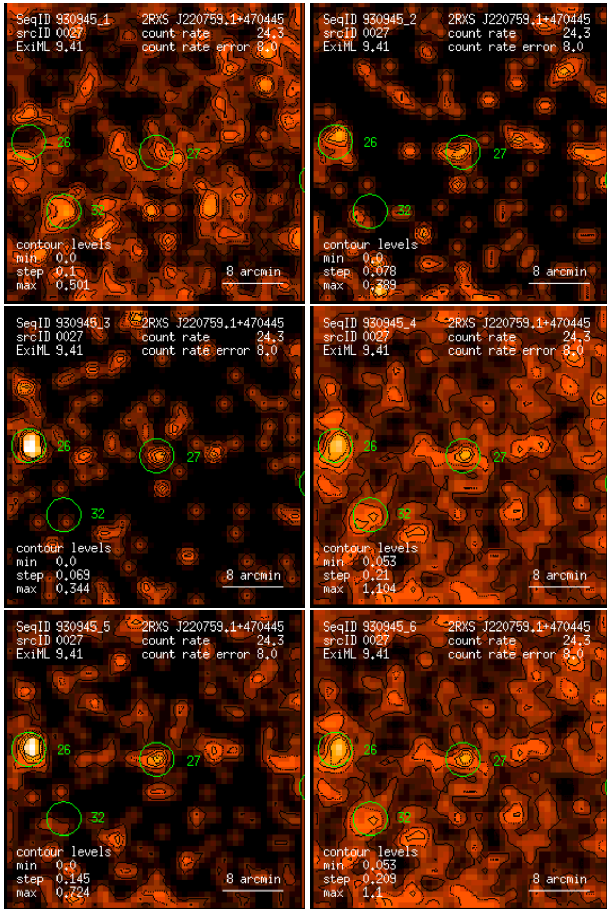
Figure 27: RASS 930945: detection 0027: band rate images, Gaussian filter: (1) PSPC channels 11 – 41, (2) 52 – 90, (3) 91 – 201, (4) 11 – 235, (5) 52 – 201, (6) 11 – 201. Broad band rates in counts/ks. Band rate contour levels in counts/ks/arcmin 2 .
