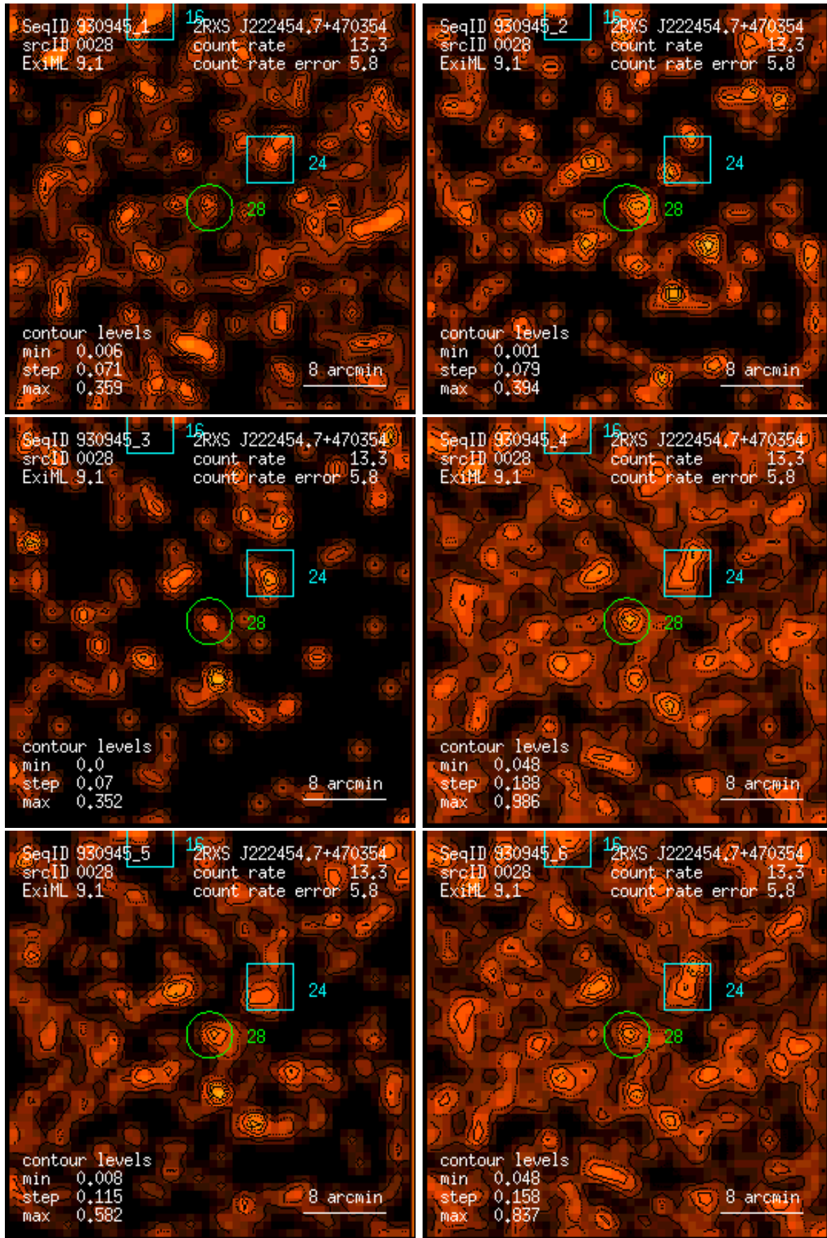
Figure 28: RASS 930945: detection 0028: band rate images, Gaussian filter: (1) PSPC channels 11 – 41, (2) 52 – 90, (3) 91 – 201, (4) 11 – 235, (5) 52 – 201, (6) 11 – 201. Broad band rates in counts/ks. Band rate contour levels in counts/ks/arcmin 2 .
