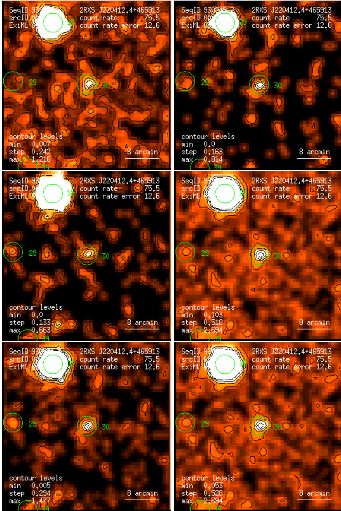
Figure 30: RASS 930945: detection 0030: band rate images, Gaussian filter: (1) PSPC channels 11 – 41, (2) 52 – 90, (3) 91 – 201, (4) 11 – 235, (5) 52 – 201, (6) 11 – 201. Broad band rates in counts/ks. Band rate contour levels in counts/ks/arcmin 2 .
