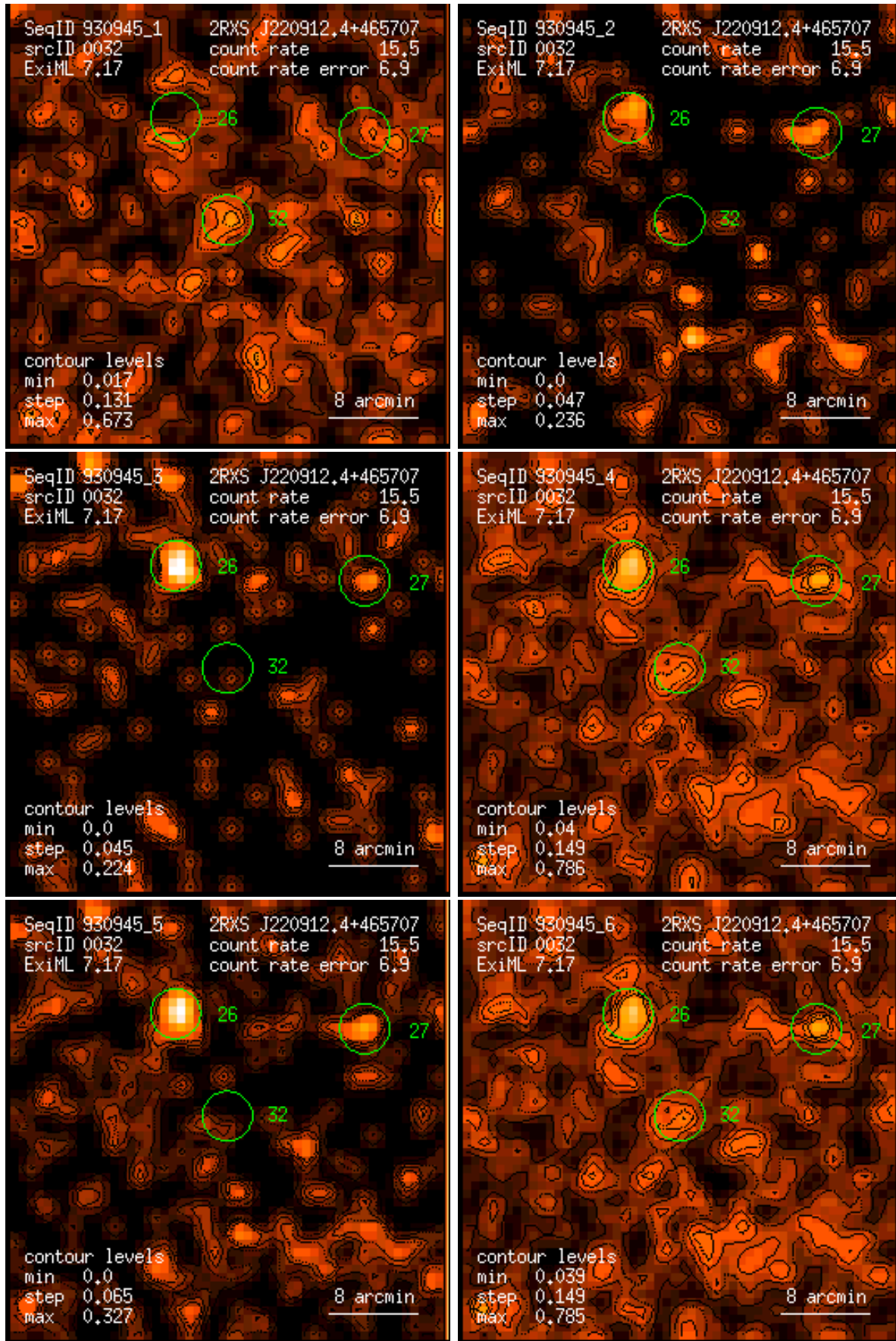
Figure 32: RASS 930945: detection 0032: band rate images, Gaussian filter: (1) PSPC channels 11 – 41, (2) 52 – 90, (3) 91 – 201, (4) 11 – 235, (5) 52 – 201, (6) 11 – 201. Broad band rates in counts/ks. Band rate contour levels in counts/ks/arcmin 2 .
