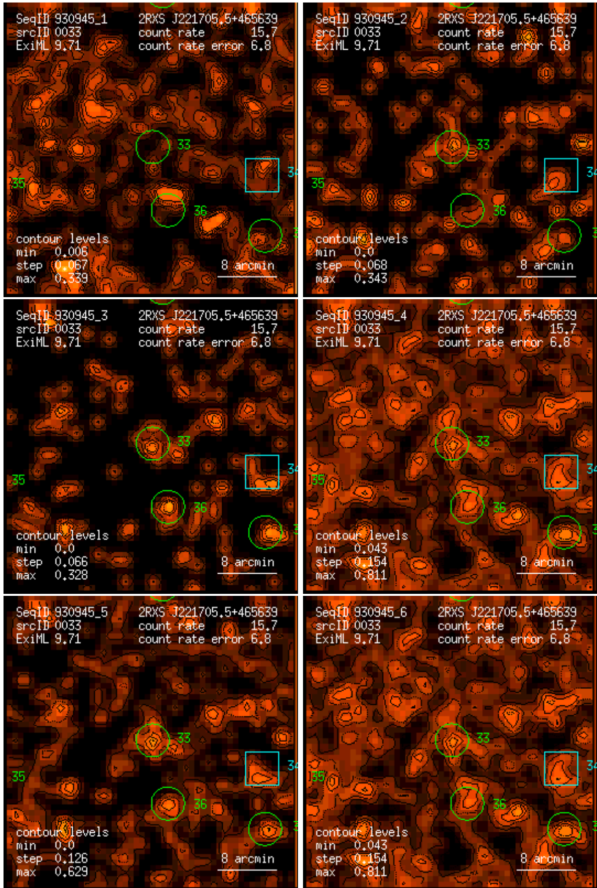
Figure 33: RASS 930945: detection 0033: band rate images, Gaussian filter: (1) PSPC channels 11 – 41, (2) 52 – 90, (3) 91 – 201, (4) 11 – 235, (5) 52 – 201, (6) 11 – 201. Broad band rates in counts/ks. Band rate contour levels in counts/ks/arcmin 2 .
