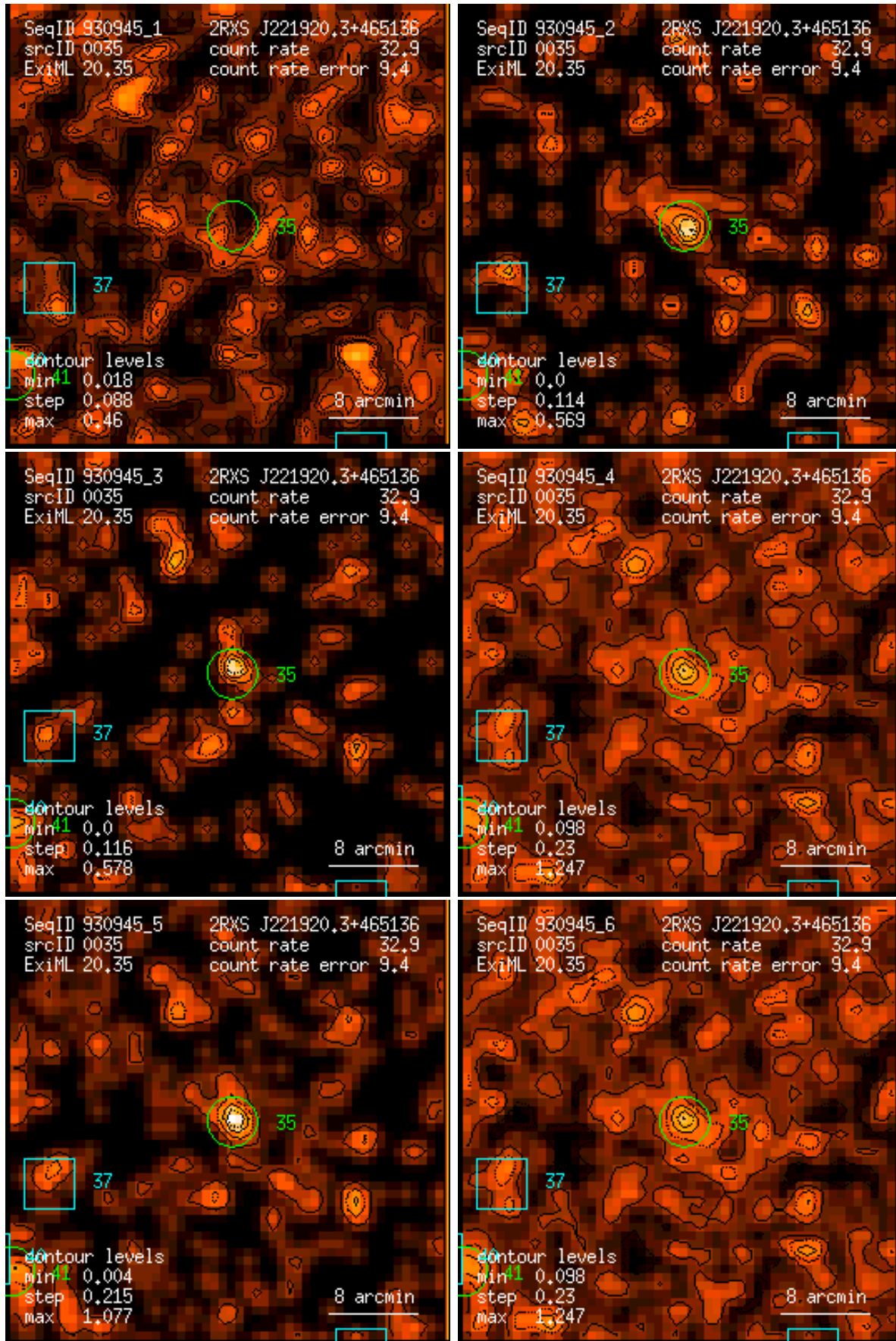
Figure 35: RASS 930945: detection 0035: band rate images, Gaussian filter: (1) PSPC channels 11 – 41, (2) 52 – 90, (3) 91 – 201, (4) 11 – 235, (5) 52 – 201, (6) 11 – 201. Broad band rates in counts/ks. Band rate contour levels in counts/ks/arcmin 2 .
