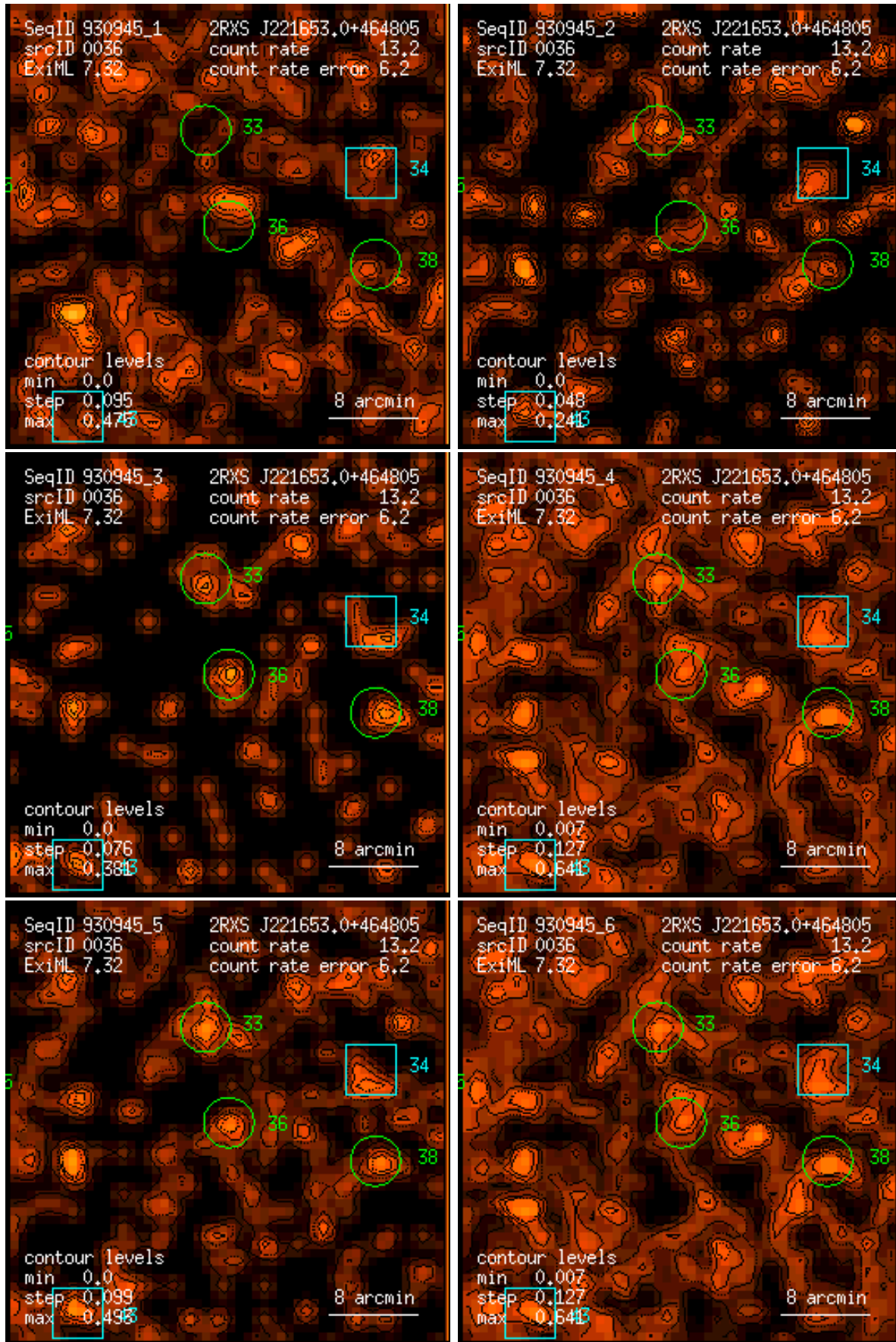
Figure 36: RASS 930945: detection 0036: band rate images, Gaussian filter: (1) PSPC channels 11 – 41, (2) 52 – 90, (3) 91 – 201, (4) 11 – 235, (5) 52 – 201, (6) 11 – 201. Broad band rates in counts/ks. Band rate contour levels in counts/ks/arcmin 2 .
