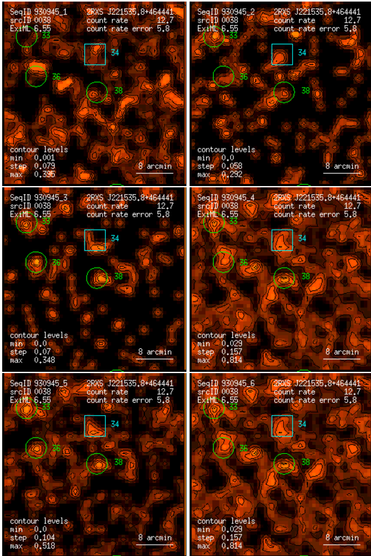
Figure 38: RASS 930945: detection 0038: band rate images, Gaussian filter: (1) PSPC channels 11 – 41, (2) 52 – 90, (3) 91 – 201, (4) 11 – 235, (5) 52 – 201, (6) 11 – 201. Broad band rates in counts/ks. Band rate contour levels in counts/ks/arcmin 2 .
