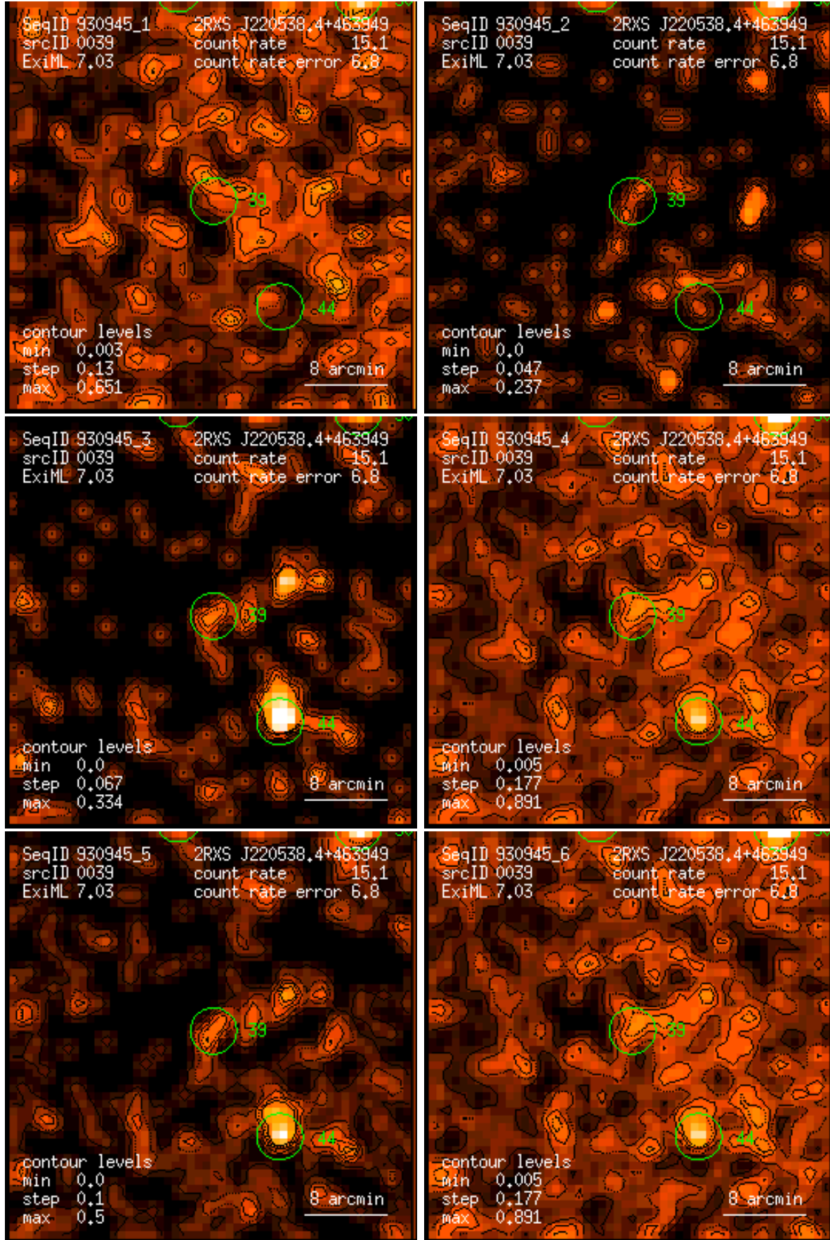
Figure 39: RASS 930945: detection 0039: band rate images, Gaussian filter: (1) PSPC channels 11 – 41, (2) 52 – 90, (3) 91 – 201, (4) 11 – 235, (5) 52 – 201, (6) 11 – 201. Broad band rates in counts/ks. Band rate contour levels in counts/ks/arcmin 2 .
