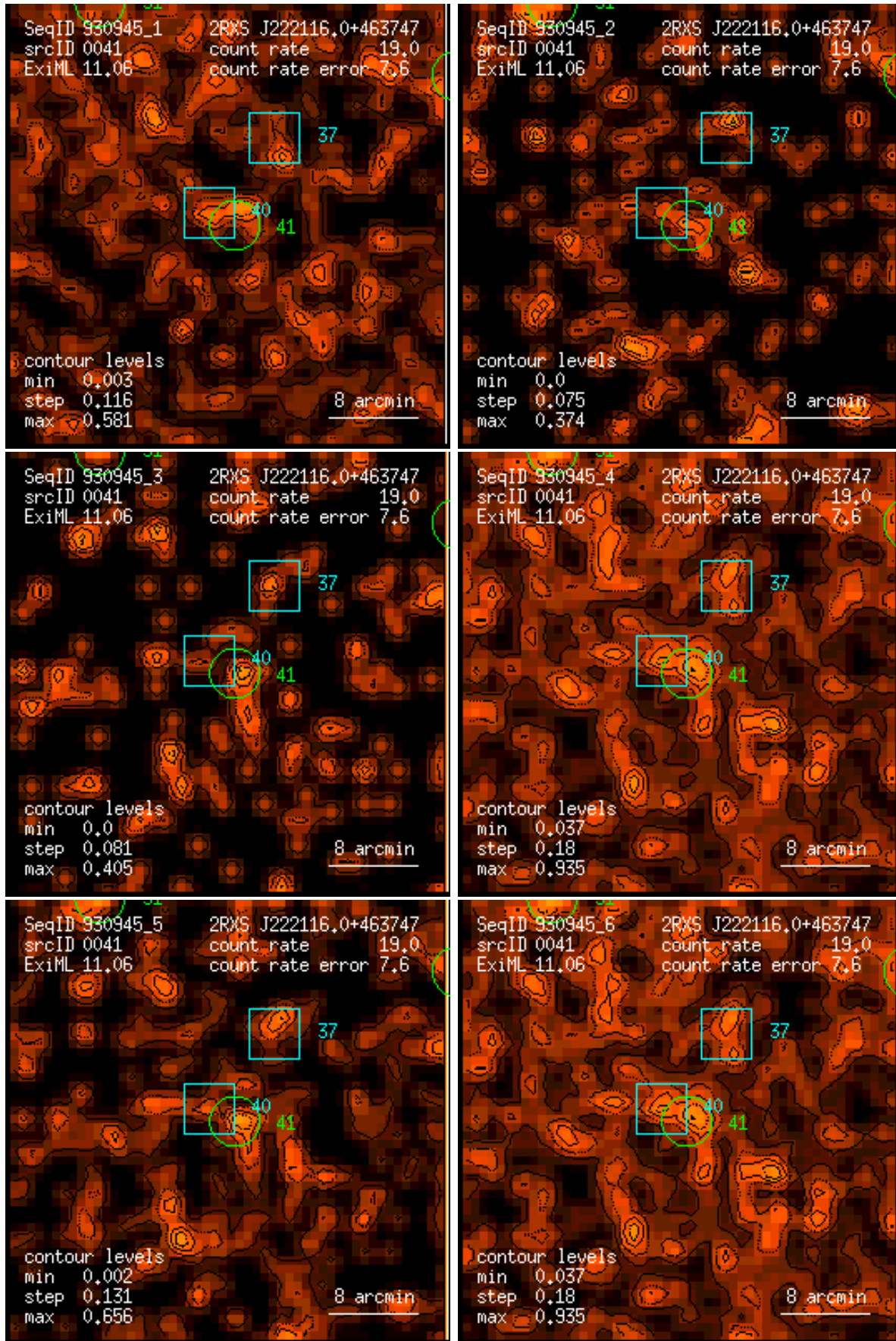
Figure 41: RASS 930945: detection 0041: band rate images, Gaussian filter: (1) PSPC channels 11 – 41, (2) 52 – 90, (3) 91 – 201, (4) 11 – 235, (5) 52 – 201, (6) 11 – 201. Broad band rates in counts/ks. Band rate contour levels in counts/ks/arcmin 2 .
