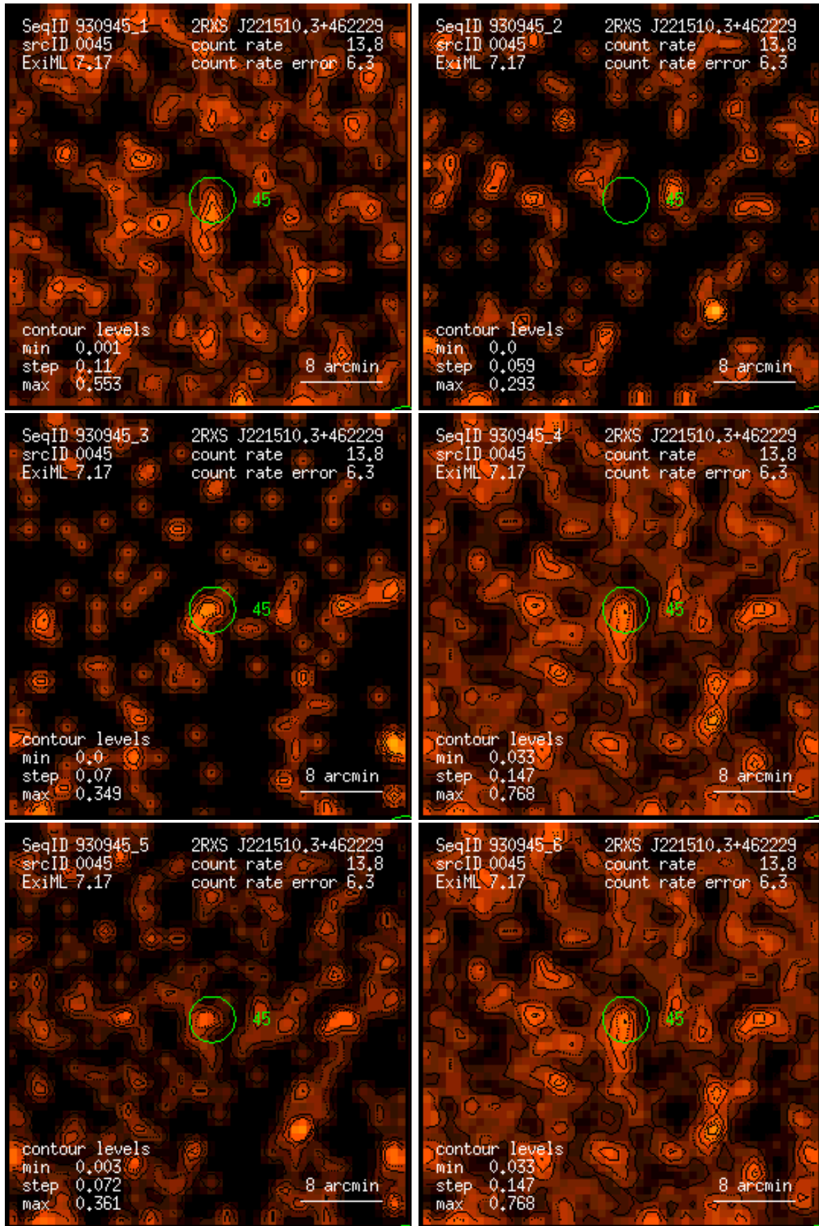
Figure 45: RASS 930945: detection 0045: band rate images, Gaussian filter: (1) PSPC channels 11 – 41, (2) 52 – 90, (3) 91 – 201, (4) 11 – 235, (5) 52 – 201, (6) 11 – 201. Broad band rates in counts/ks. Band rate contour levels in counts/ks/arcmin 2 .
