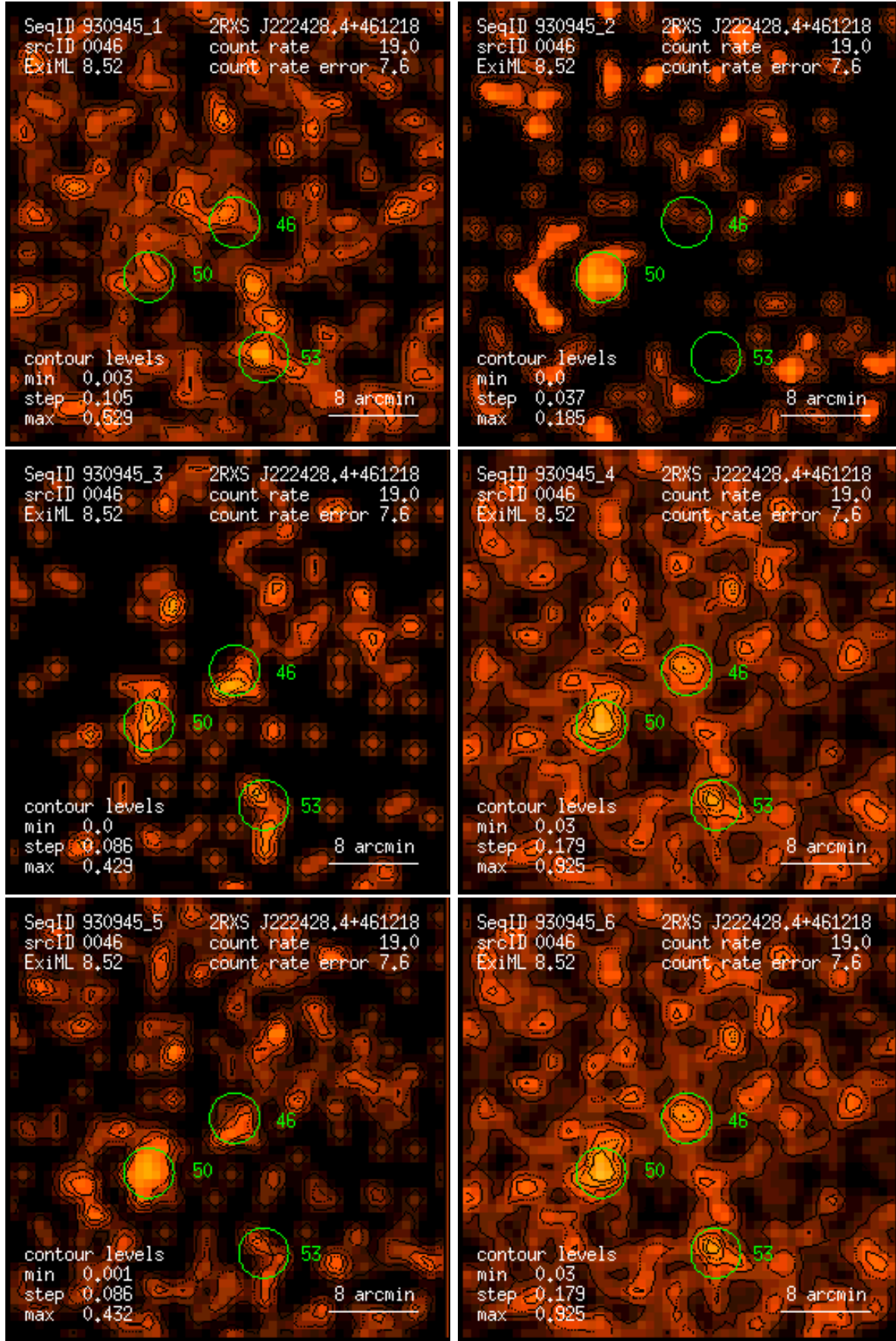
Figure 46: RASS 930945: detection 0046: band rate images, Gaussian filter: (1) PSPC channels 11 – 41, (2) 52 – 90, (3) 91 – 201, (4) 11 – 235, (5) 52 – 201, (6) 11 – 201. Broad band rates in counts/ks. Band rate contour levels in counts/ks/arcmin 2 .
