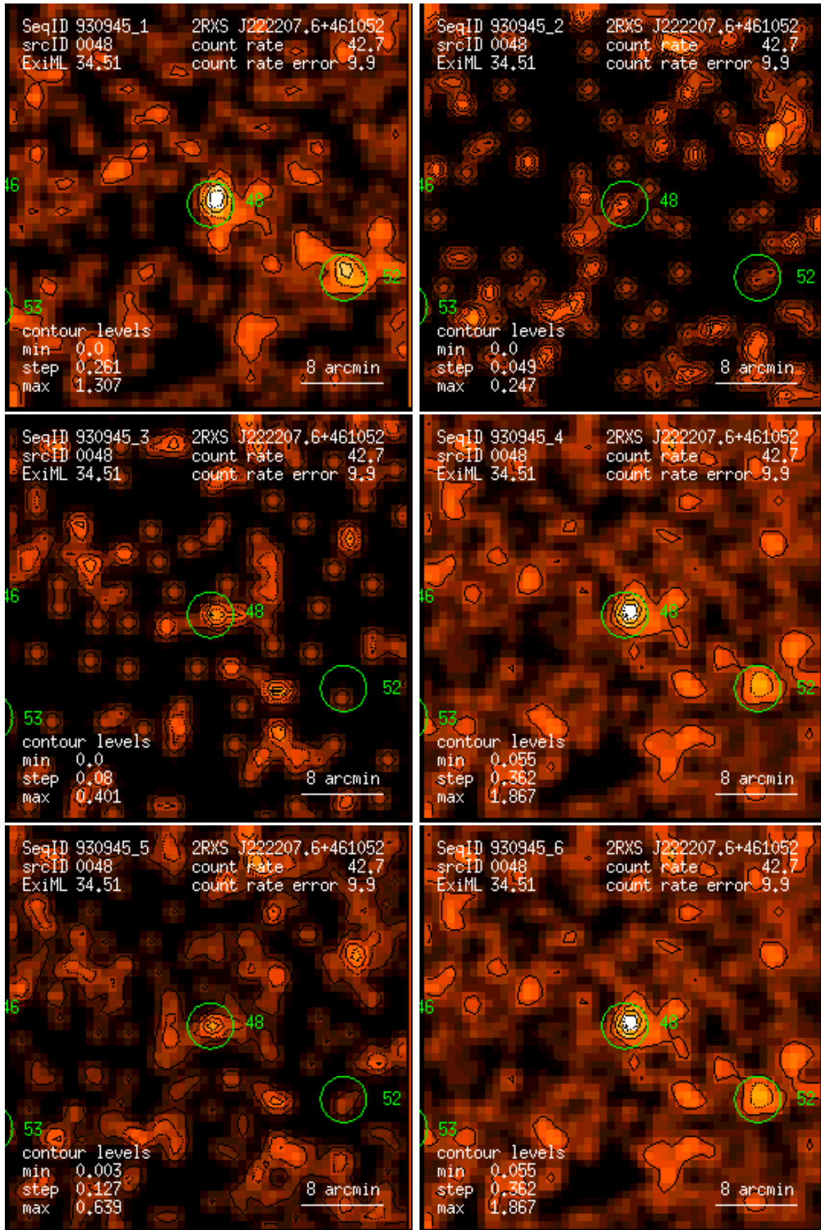
Figure 48: RASS 930945: detection 0048: band rate images, Gaussian filter: (1) PSPC channels 11 – 41, (2) 52 – 90, (3) 91 – 201, (4) 11 – 235, (5) 52 – 201, (6) 11 – 201. Broad band rates in counts/ks. Band rate contour levels in counts/ks/arcmin 2 .
