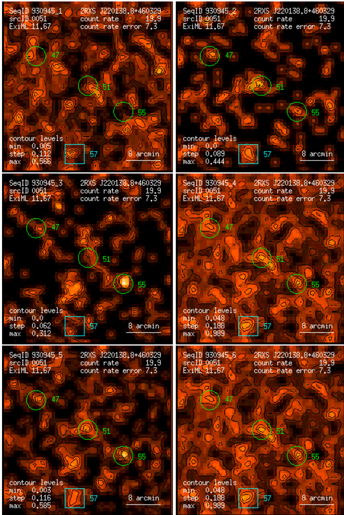
Figure 51: RASS 930945: detection 0051: band rate images, Gaussian filter: (1) PSPC channels 11 – 41, (2) 52 – 90, (3) 91 – 201, (4) 11 – 235, (5) 52 – 201, (6) 11 – 201. Broad band rates in counts/ks. Band rate contour levels in counts/ks/arcmin 2 .
