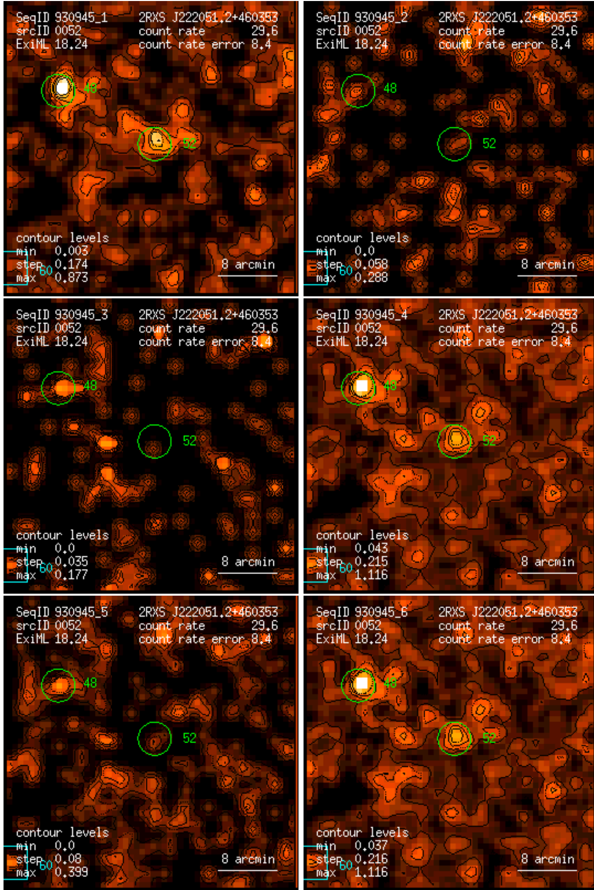
Figure 52: RASS 930945: detection 0052: band rate images, Gaussian filter: (1) PSPC channels 11 – 41, (2) 52 – 90, (3) 91 – 201, (4) 11 – 235, (5) 52 – 201, (6) 11 – 201. Broad band rates in counts/ks. Band rate contour levels in counts/ks/arcmin 2 .
