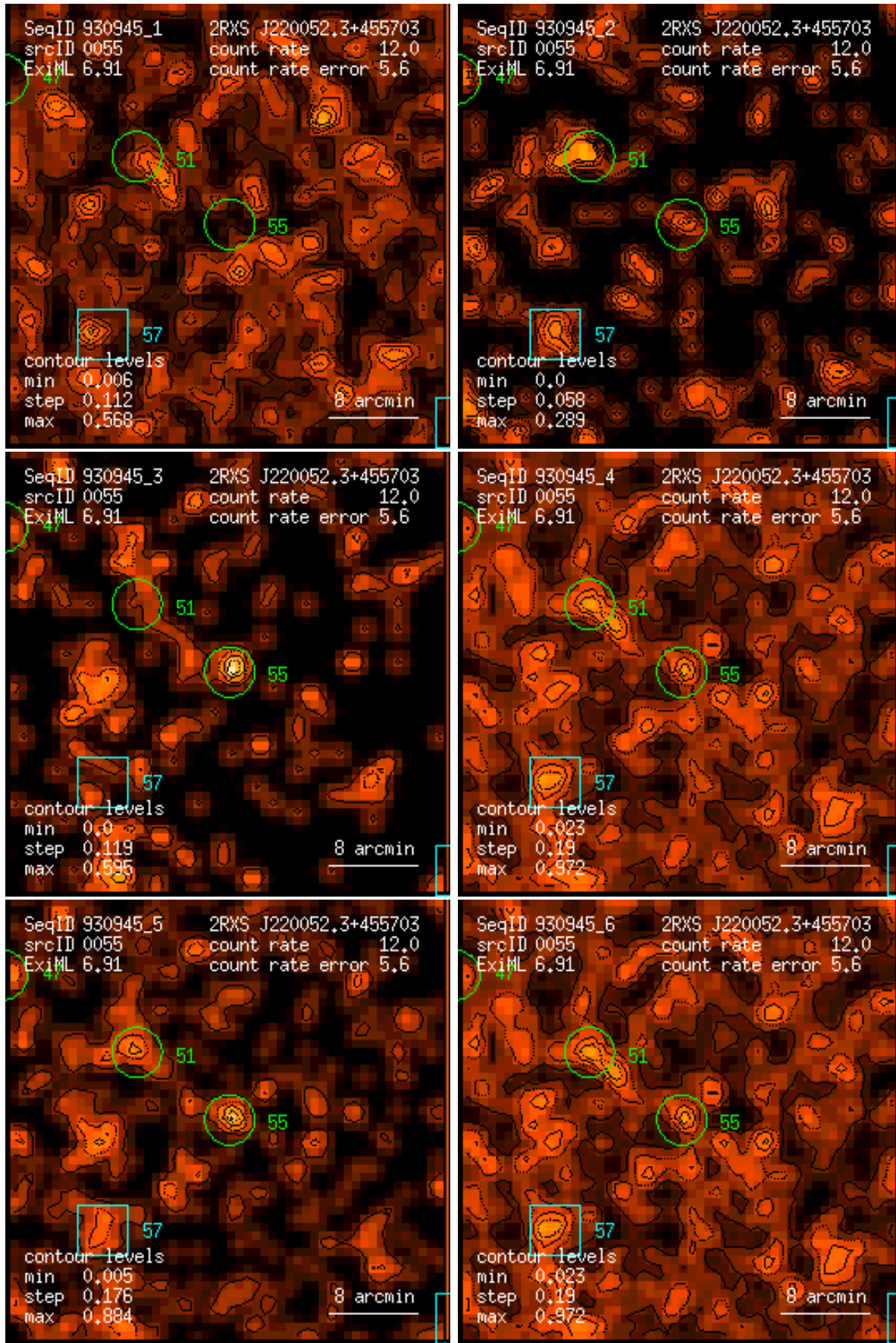
Figure 55: RASS 930945: detection 0055: band rate images, Gaussian filter: (1) PSPC channels 11 – 41, (2) 52 – 90, (3) 91 – 201, (4) 11 – 235, (5) 52 – 201, (6) 11 – 201. Broad band rates in counts/ks. Band rate contour levels in counts/ks/arcmin 2 .
