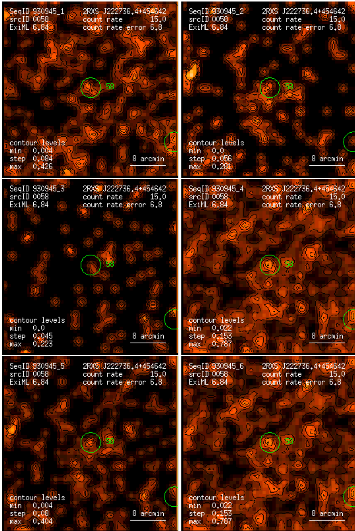
Figure 58: RASS 930945: detection 0058: band rate images, Gaussian filter: (1) PSPC channels 11 – 41, (2) 52 – 90, (3) 91 – 201, (4) 11 – 235, (5) 52 – 201, (6) 11 – 201. Broad band rates in counts/ks. Band rate contour levels in counts/ks/arcmin 2 .
