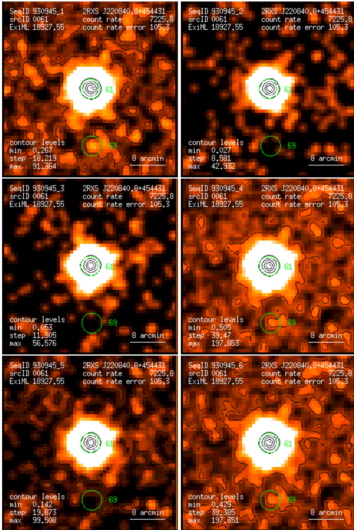
Figure 61: RASS 930945: detection 0061: band rate images, Gaussian filter: (1) PSPC channels 11 – 41, (2) 52 – 90, (3) 91 – 201, (4) 11 – 235, (5) 52 – 201, (6) 11 – 201. Broad band rates in counts/ks. Band rate contour levels in counts/ks/arcmin 2 .
