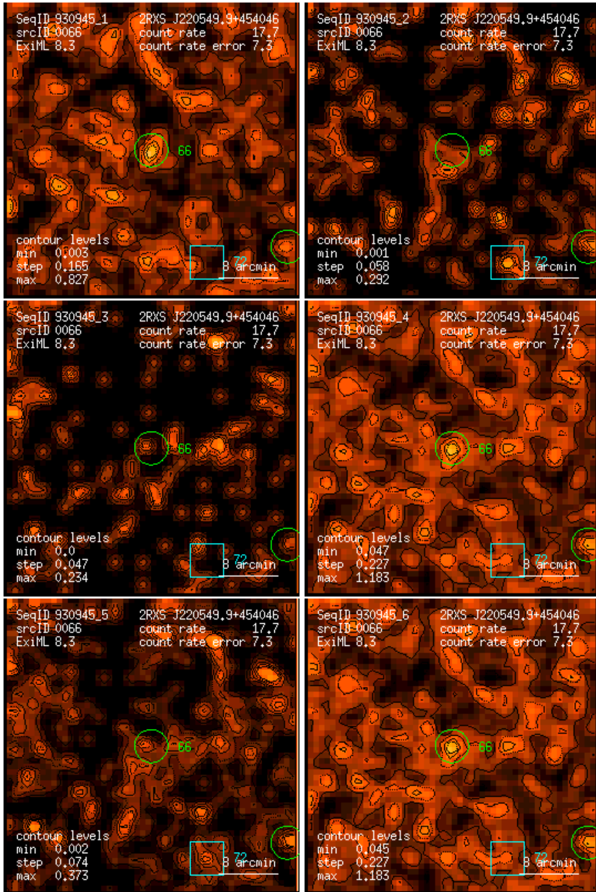
Figure 66: RASS 930945: detection 0066: band rate images, Gaussian filter: (1) PSPC channels 11 – 41, (2) 52 – 90, (3) 91 – 201, (4) 11 – 235, (5) 52 – 201, (6) 11 – 201. Broad band rates in counts/ks. Band rate contour levels in counts/ks/arcmin 2 .
