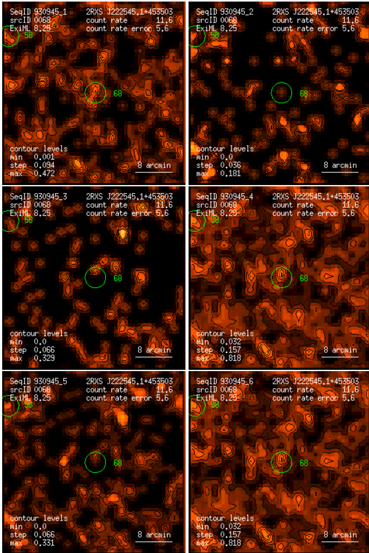
Figure 68: RASS 930945: detection 0068: band rate images, Gaussian filter: (1) PSPC channels 11 – 41, (2) 52 – 90, (3) 91 – 201, (4) 11 – 235, (5) 52 – 201, (6) 11 – 201. Broad band rates in counts/ks. Band rate contour levels in counts/ks/arcmin 2 .
