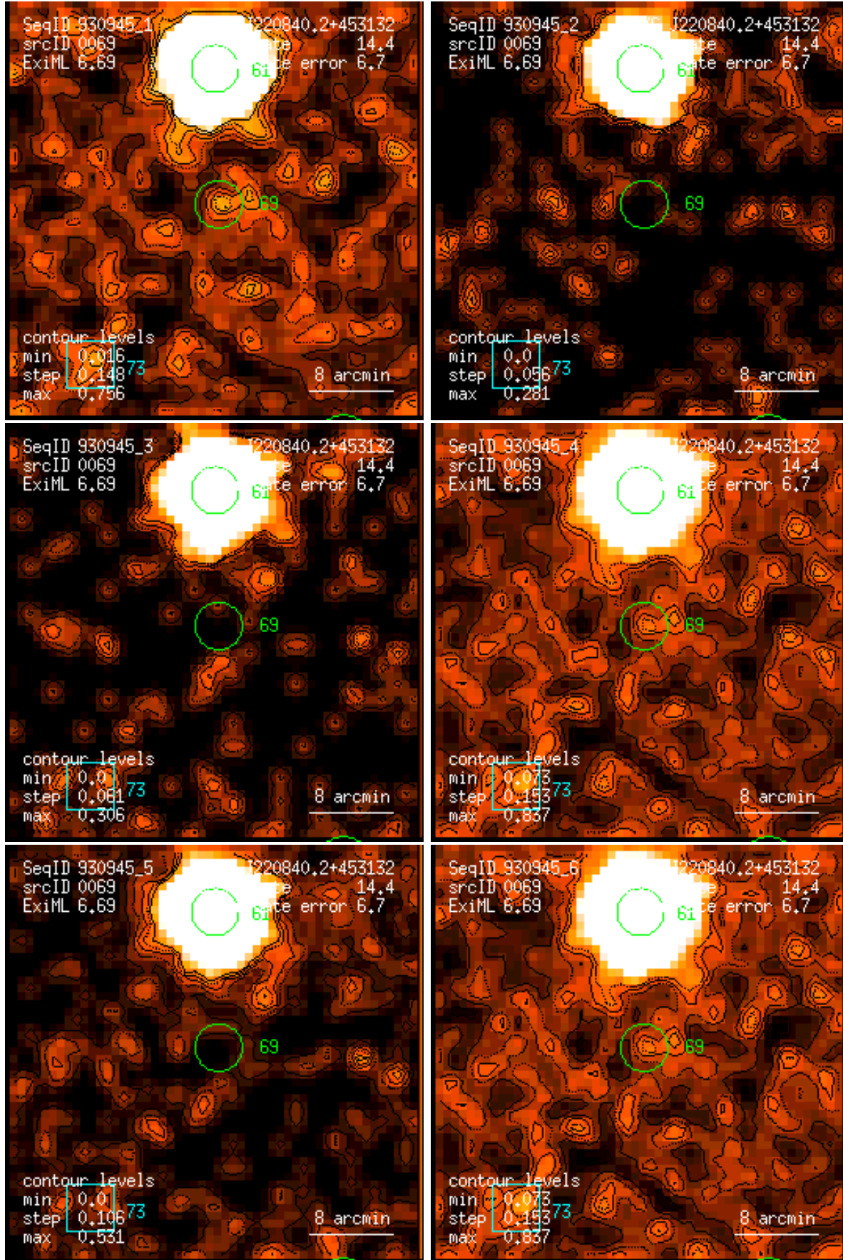
Figure 69: RASS 930945: detection 0069: band rate images, Gaussian filter: (1) PSPC channels 11 – 41, (2) 52 – 90, (3) 91 – 201, (4) 11 – 235, (5) 52 – 201, (6) 11 – 201. Broad band rates in counts/ks. Band rate contour levels in counts/ks/arcmin 2 .
