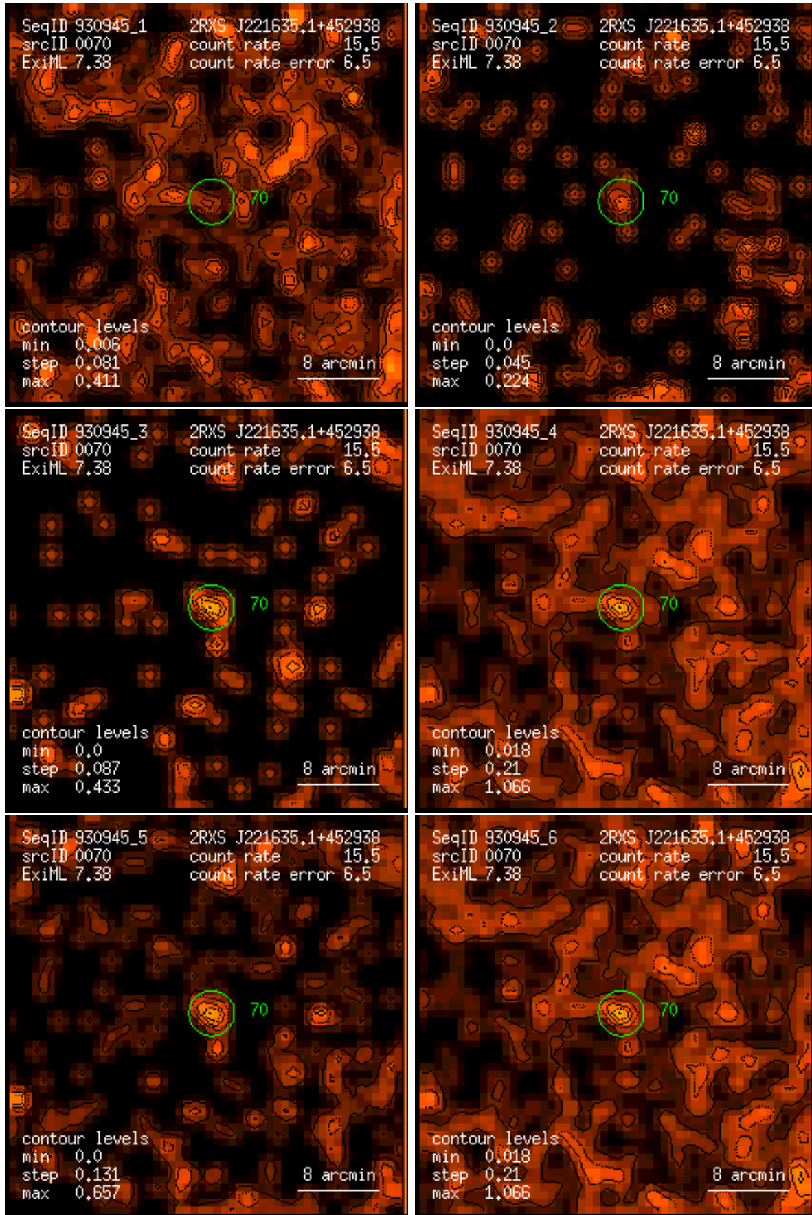
Figure 70: RASS 930945: detection 0070: band rate images, Gaussian filter: (1) PSPC channels 11 – 41, (2) 52 – 90, (3) 91 – 201, (4) 11 – 235, (5) 52 – 201, (6) 11 – 201. Broad band rates in counts/ks. Band rate contour levels in counts/ks/arcmin 2 .
