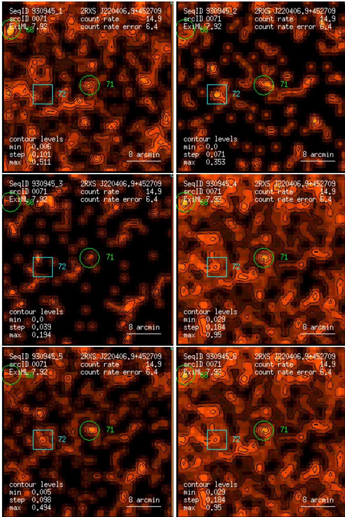
Figure 71: RASS 930945: detection 0071: band rate images, Gaussian filter: (1) PSPC channels 11 – 41, (2) 52 – 90, (3) 91 – 201, (4) 11 – 235, (5) 52 – 201, (6) 11 – 201. Broad band rates in counts/ks. Band rate contour levels in counts/ks/arcmin 2 .
