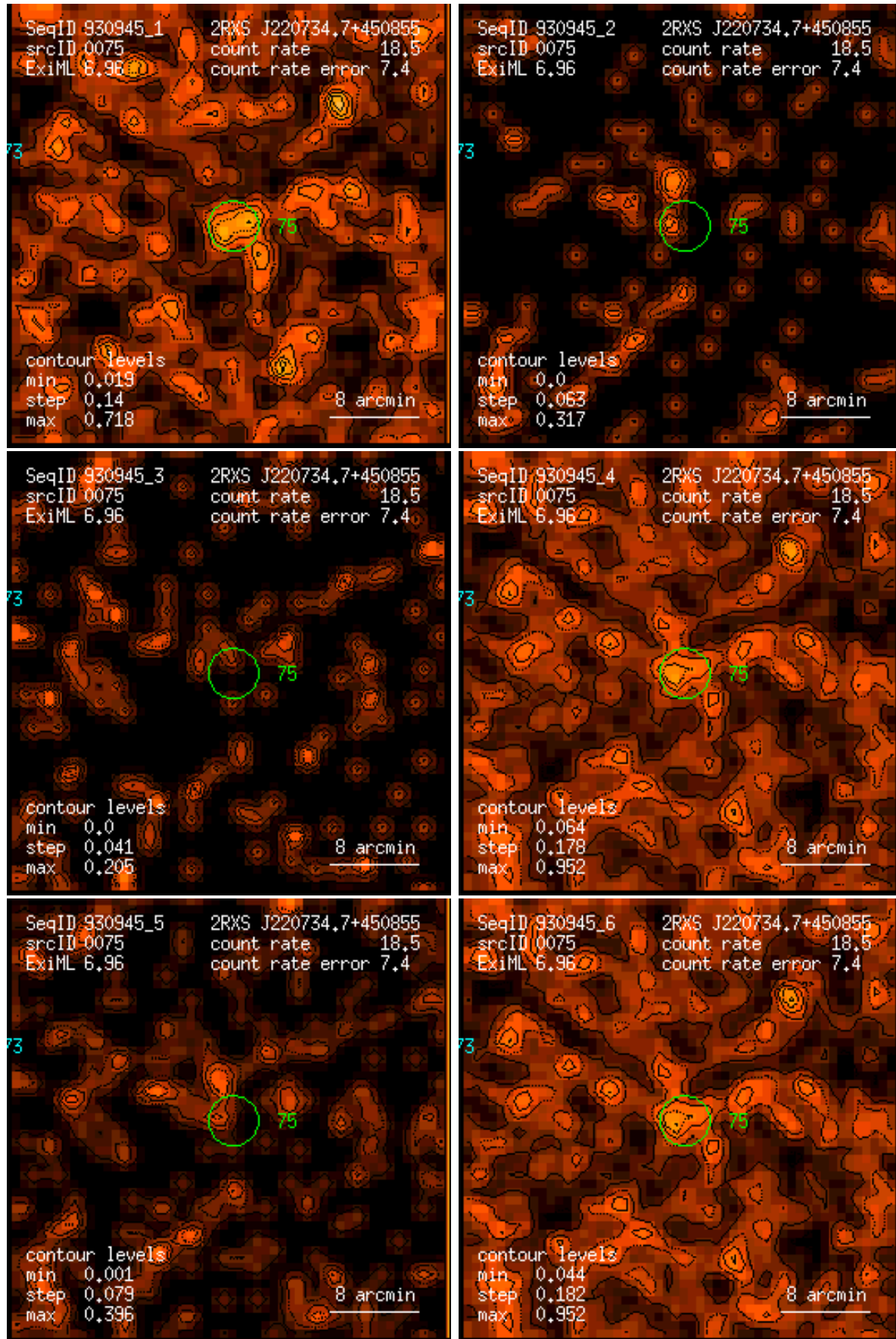
Figure 75: RASS 930945: detection 0075: band rate images, Gaussian filter: (1) PSPC channels 11 – 41, (2) 52 – 90, (3) 91 – 201, (4) 11 – 235, (5) 52 – 201, (6) 11 – 201. Broad band rates in counts/ks. Band rate contour levels in counts/ks/arcmin 2 .
