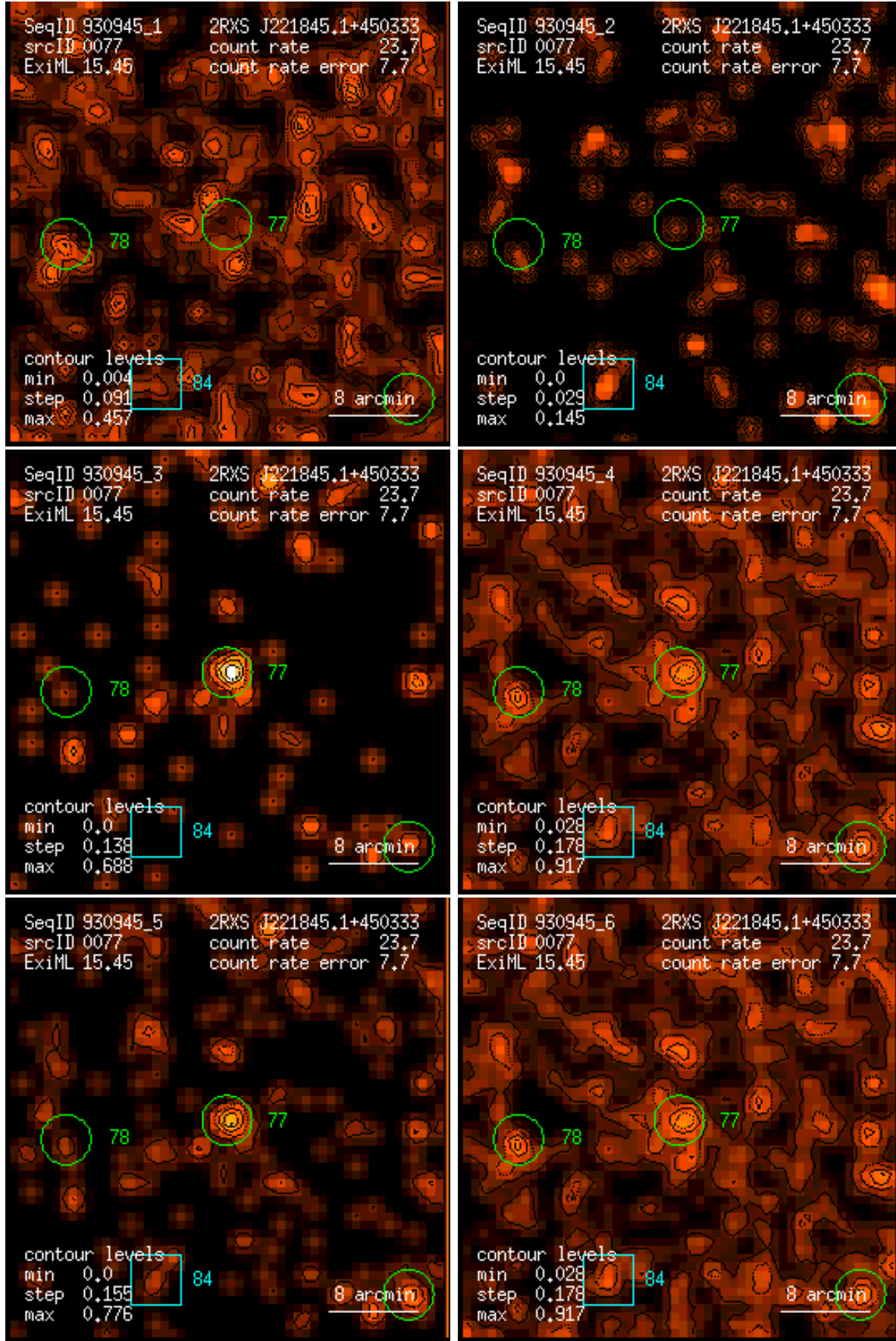
Figure 77: RASS 930945: detection 0077: band rate images, Gaussian filter: (1) PSPC channels 11 – 41, (2) 52 – 90, (3) 91 – 201, (4) 11 – 235, (5) 52 – 201, (6) 11 – 201. Broad band rates in counts/ks. Band rate contour levels in counts/ks/arcmin 2 .
