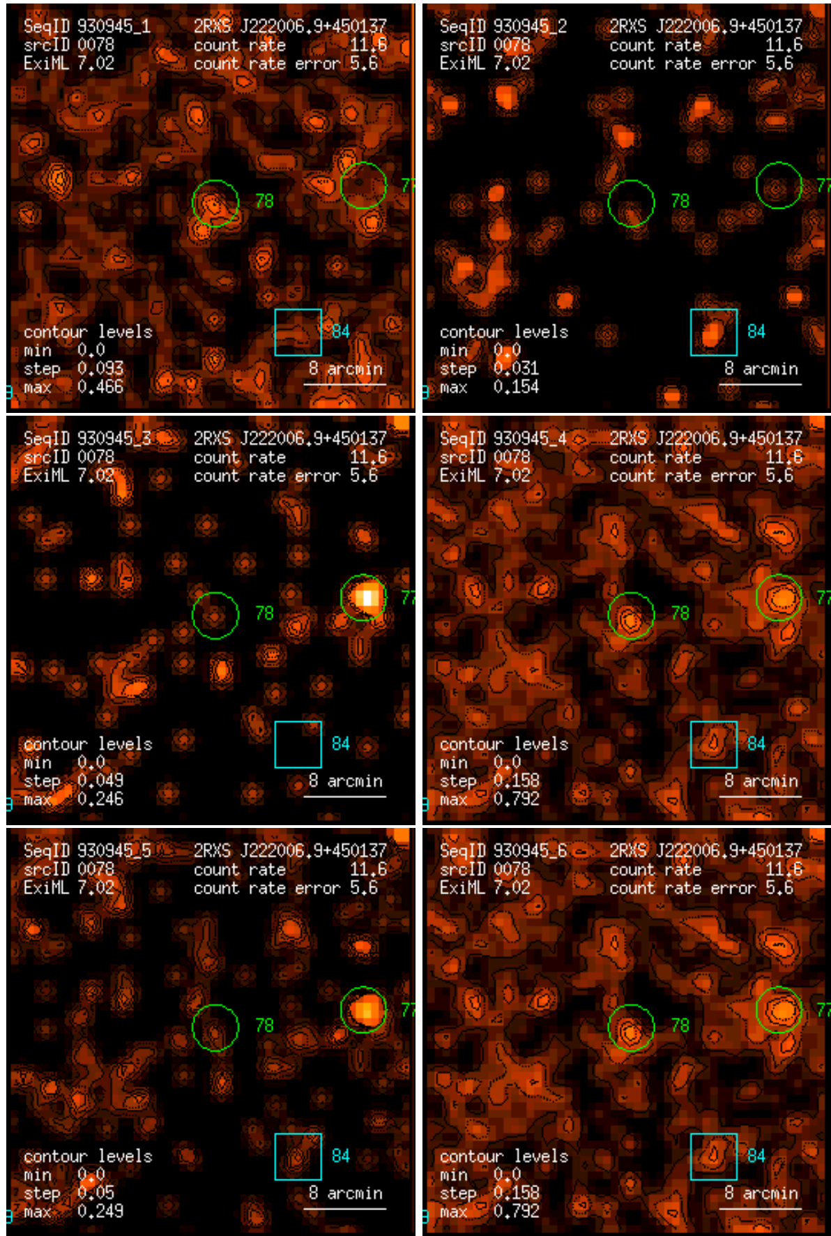
Figure 78: RASS 930945: detection 0078: band rate images, Gaussian filter: (1) PSPC channels 11 – 41, (2) 52 – 90, (3) 91 – 201, (4) 11 – 235, (5) 52 – 201, (6) 11 – 201. Broad band rates in counts/ks. Band rate contour levels in counts/ks/arcmin 2 .
