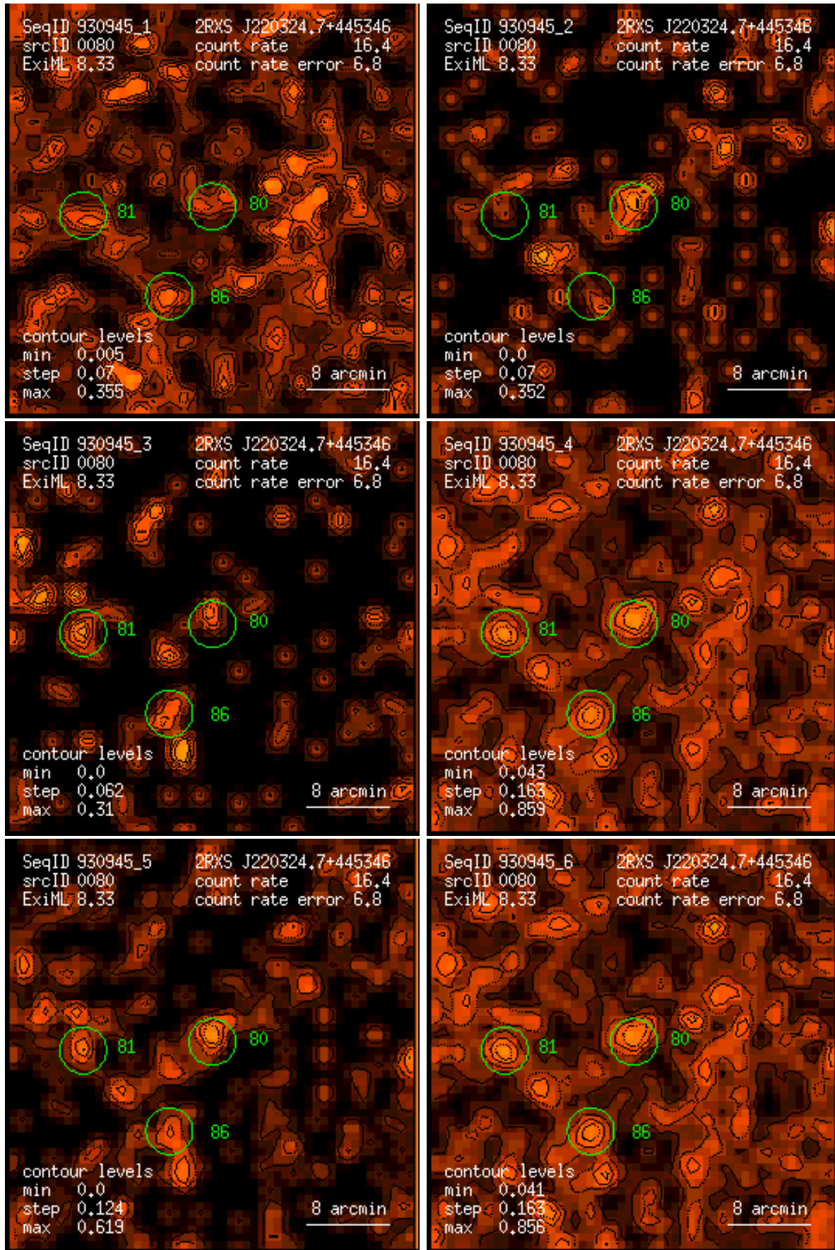
Figure 80: RASS 930945: detection 0080: band rate images, Gaussian filter: (1) PSPC channels 11 – 41, (2) 52 – 90, (3) 91 – 201, (4) 11 – 235, (5) 52 – 201, (6) 11 – 201. Broad band rates in counts/ks. Band rate contour levels in counts/ks/arcmin 2 .
