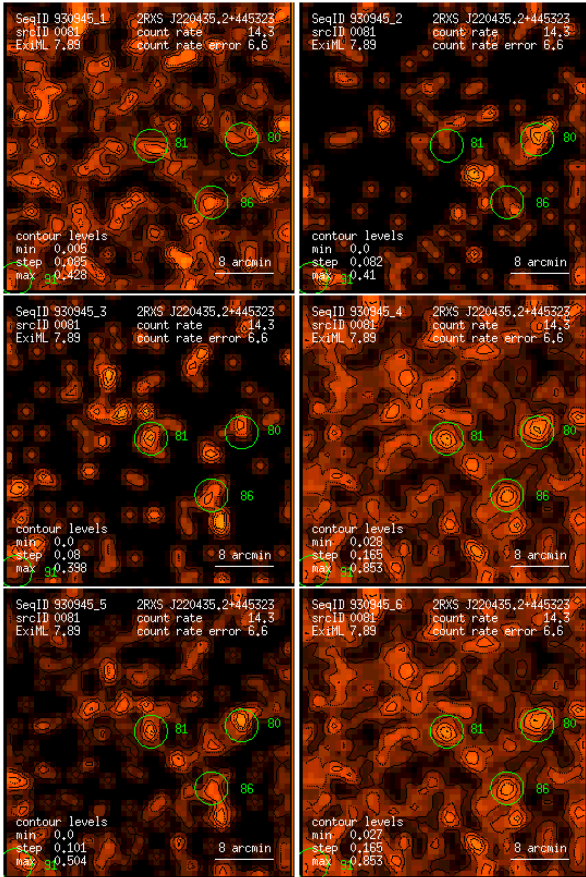
Figure 81: RASS 930945: detection 0081: band rate images, Gaussian filter: (1) PSPC channels 11 – 41, (2) 52 – 90, (3) 91 – 201, (4) 11 – 235, (5) 52 – 201, (6) 11 – 201. Broad band rates in counts/ks. Band rate contour levels in counts/ks/arcmin 2 .
