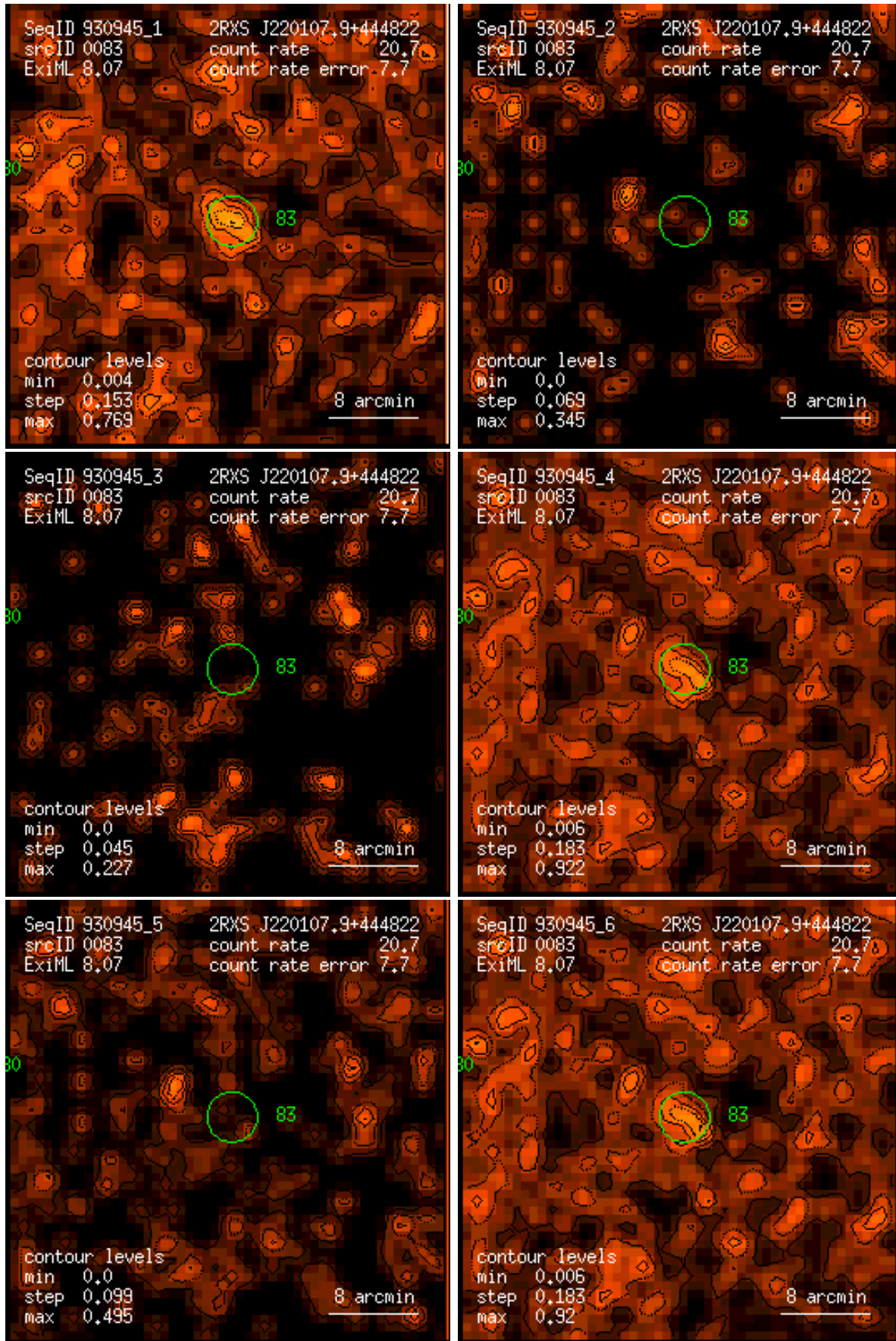
Figure 83: RASS 930945: detection 0083: band rate images, Gaussian filter: (1) PSPC channels 11 – 41, (2) 52 – 90, (3) 91 – 201, (4) 11 – 235, (5) 52 – 201, (6) 11 – 201. Broad band rates in counts/ks. Band rate contour levels in counts/ks/arcmin 2 .
