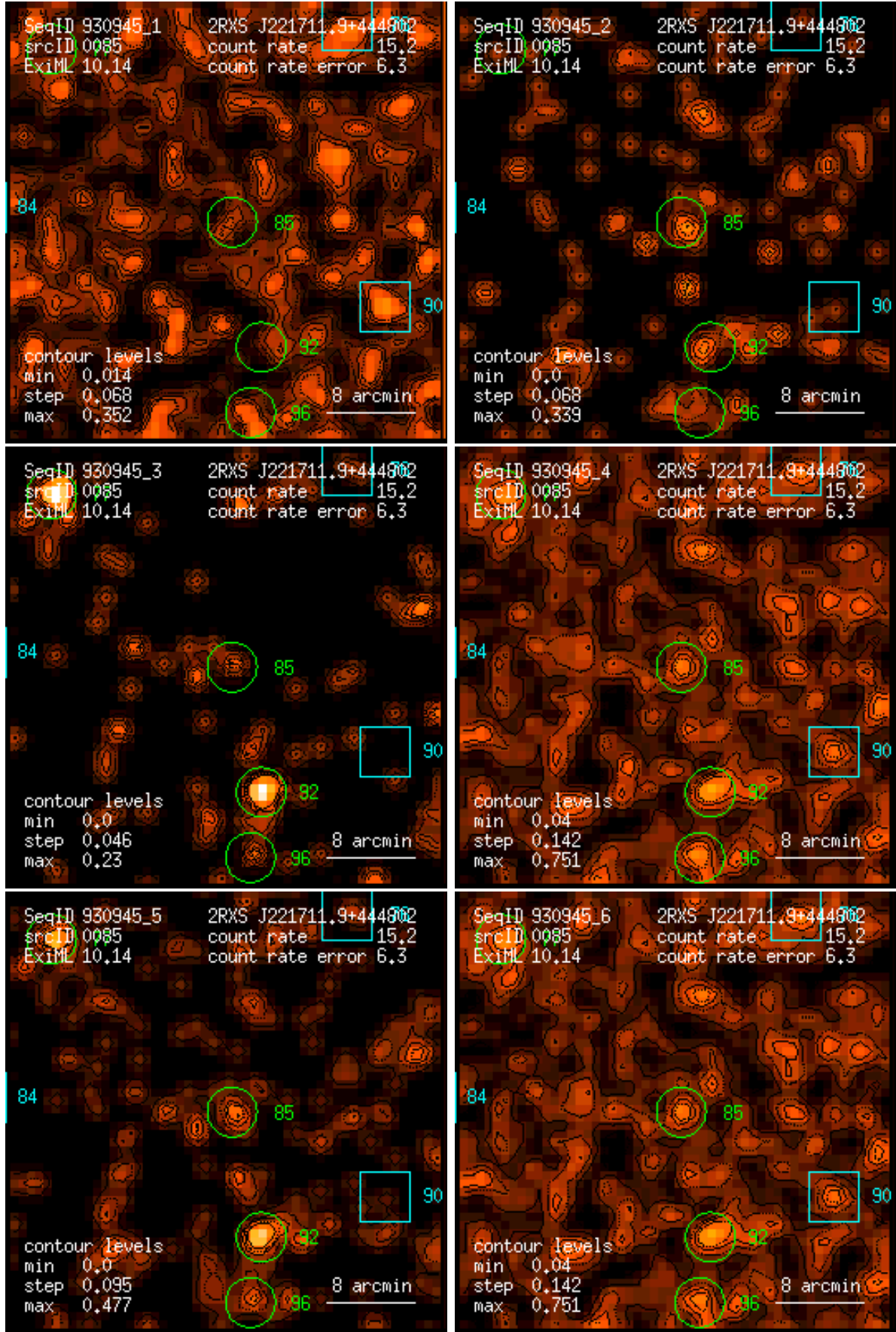
Figure 85: RASS 930945: detection 0085: band rate images, Gaussian filter: (1) PSPC channels 11 – 41, (2) 52 – 90, (3) 91 – 201, (4) 11 – 235, (5) 52 – 201, (6) 11 – 201. Broad band rates in counts/ks. Band rate contour levels in counts/ks/arcmin 2 .
