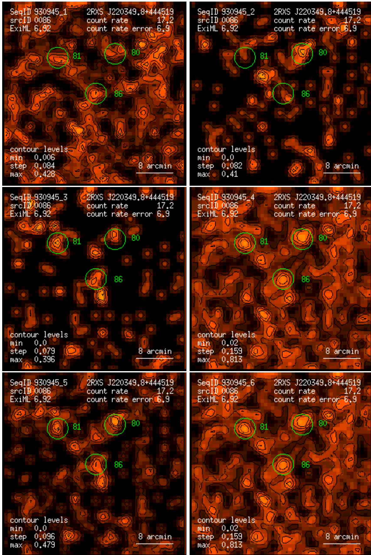
Figure 86: RASS 930945: detection 0086: band rate images, Gaussian filter: (1) PSPC channels 11 – 41, (2) 52 – 90, (3) 91 – 201, (4) 11 – 235, (5) 52 – 201, (6) 11 – 201. Broad band rates in counts/ks. Band rate contour levels in counts/ks/arcmin 2 .
