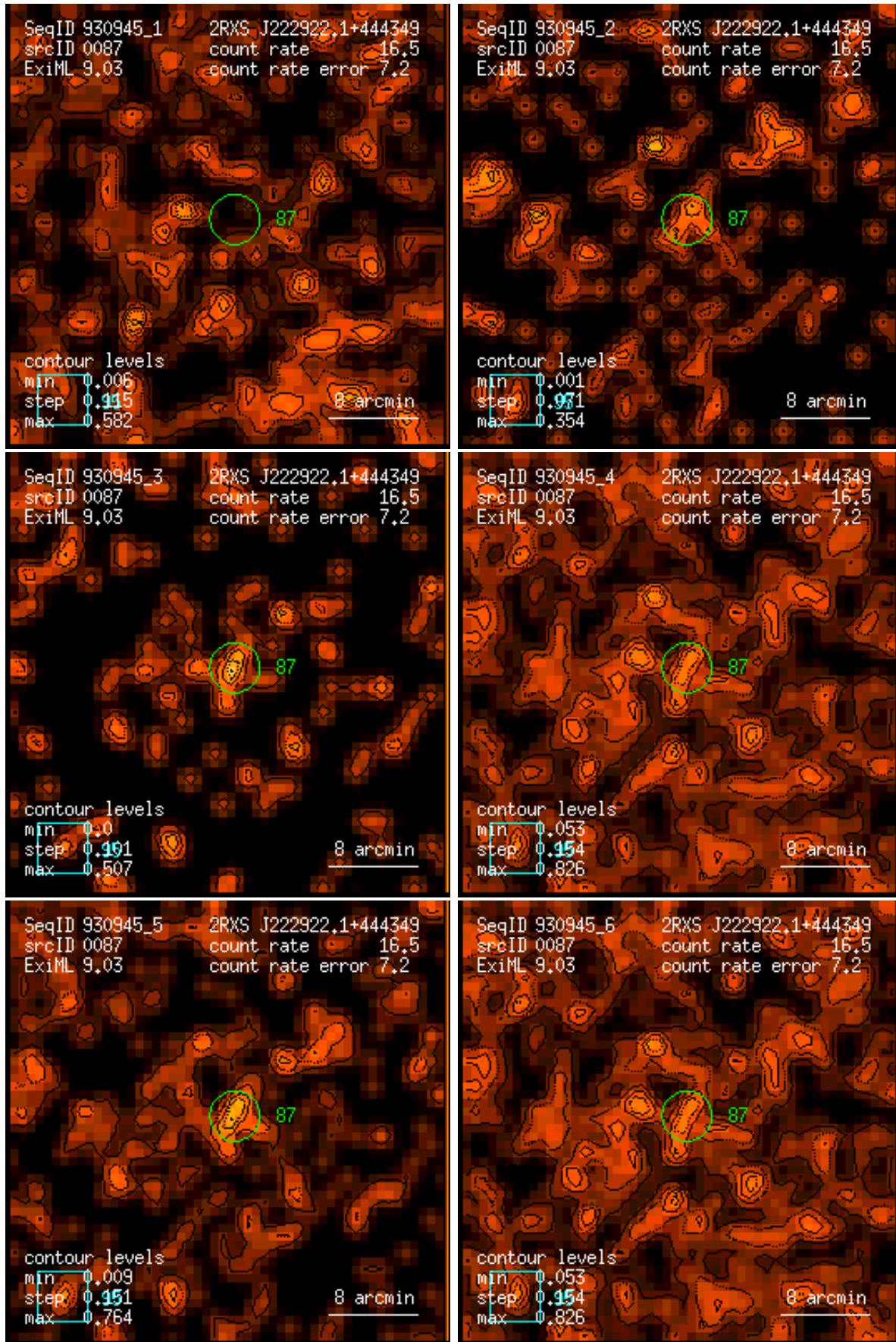
Figure 87: RASS 930945: detection 0087: band rate images, Gaussian filter: (1) PSPC channels 11 – 41, (2) 52 – 90, (3) 91 – 201, (4) 11 – 235, (5) 52 – 201, (6) 11 – 201. Broad band rates in counts/ks. Band rate contour levels in counts/ks/arcmin 2 .
