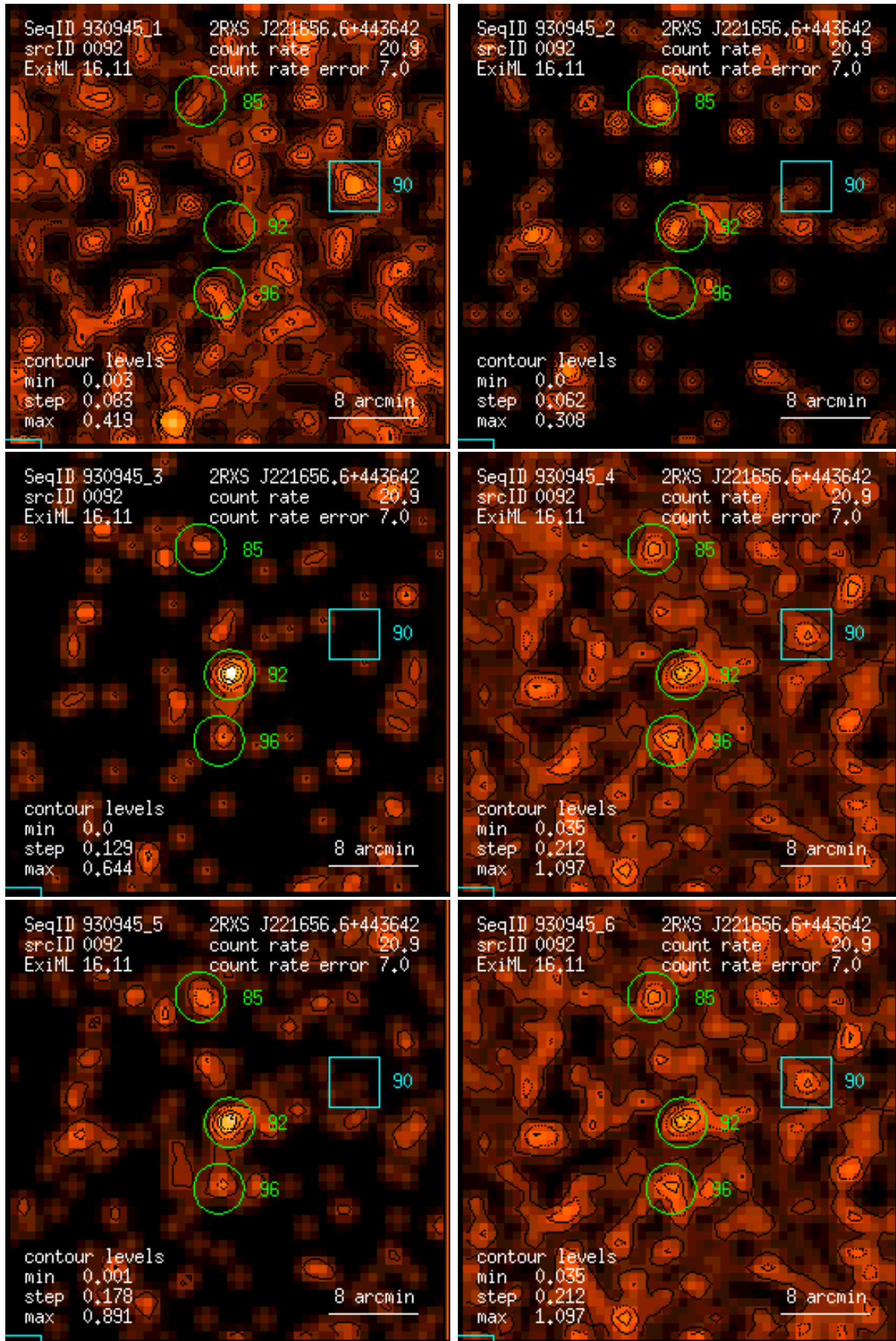
Figure 92: RASS 930945: detection 0092: band rate images, Gaussian filter: (1) PSPC channels 11 – 41, (2) 52 – 90, (3) 91 – 201, (4) 11 – 235, (5) 52 – 201, (6) 11 – 201. Broad band rates in counts/ks. Band rate contour levels in counts/ks/arcmin 2 .
