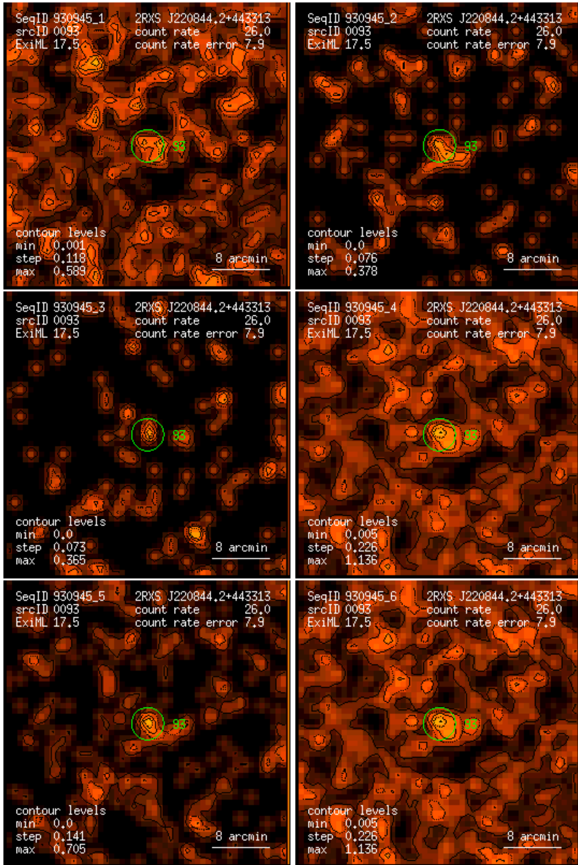
Figure 93: RASS 930945: detection 0093: band rate images, Gaussian filter: (1) PSPC channels 11 – 41, (2) 52 – 90, (3) 91 – 201, (4) 11 – 235, (5) 52 – 201, (6) 11 – 201. Broad band rates in counts/ks. Band rate contour levels in counts/ks/arcmin 2 .
