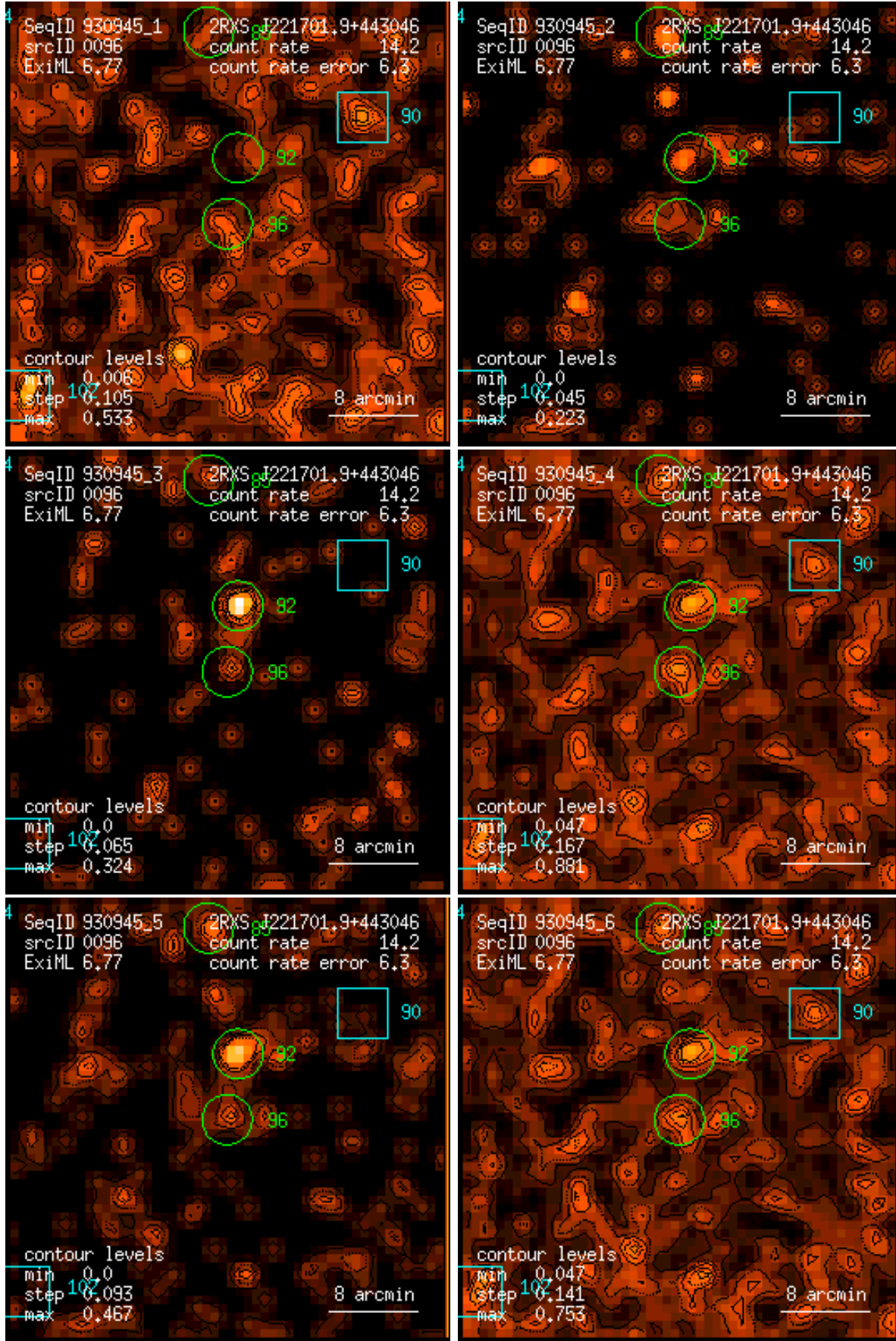
Figure 96: RASS 930945: detection 0096: band rate images, Gaussian filter: (1) PSPC channels 11 – 41, (2) 52 – 90, (3) 91 – 201, (4) 11 – 235, (5) 52 – 201, (6) 11 – 201. Broad band rates in counts/ks. Band rate contour levels in counts/ks/arcmin 2 .
