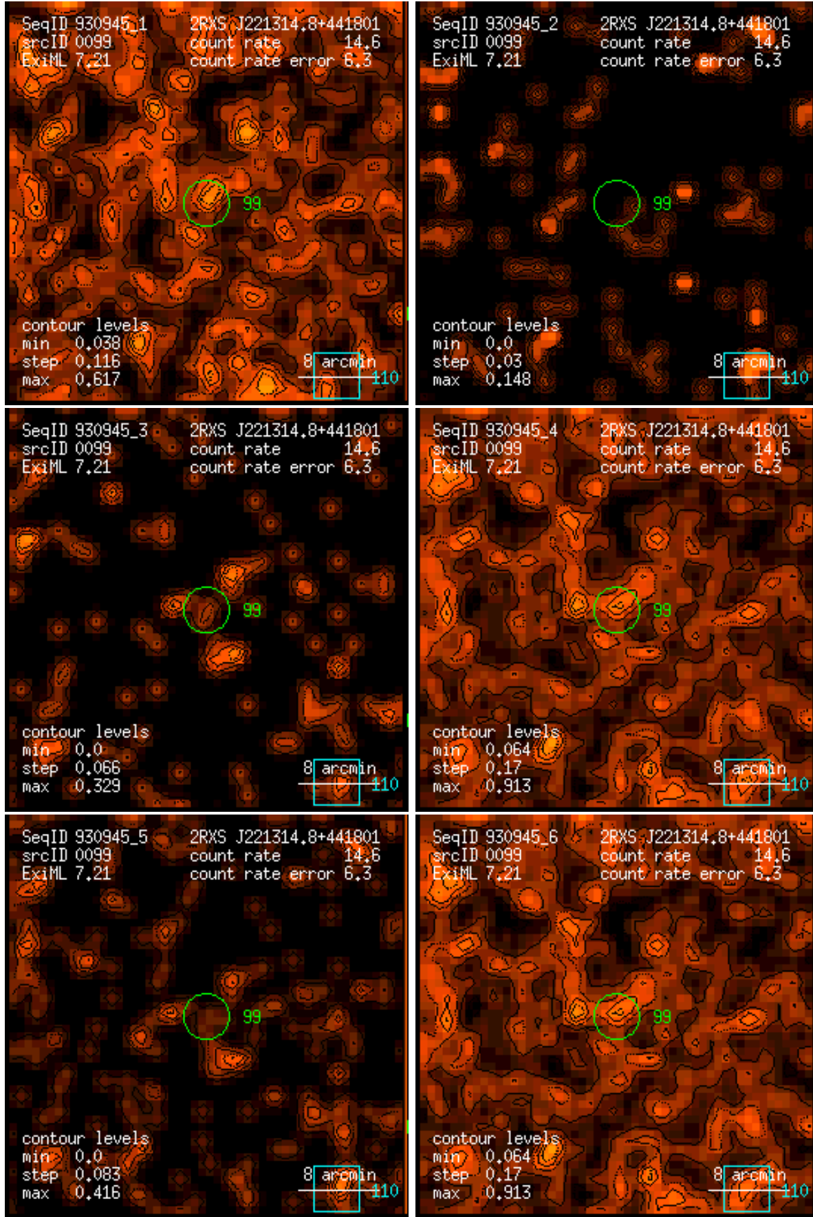
Figure 99: RASS 930945: detection 0099: band rate images, Gaussian filter: (1) PSPC channels 11 – 41, (2) 52 – 90, (3) 91 – 201, (4) 11 – 235, (5) 52 – 201, (6) 11 – 201. Broad band rates in counts/ks. Band rate contour levels in counts/ks/arcmin 2 .
