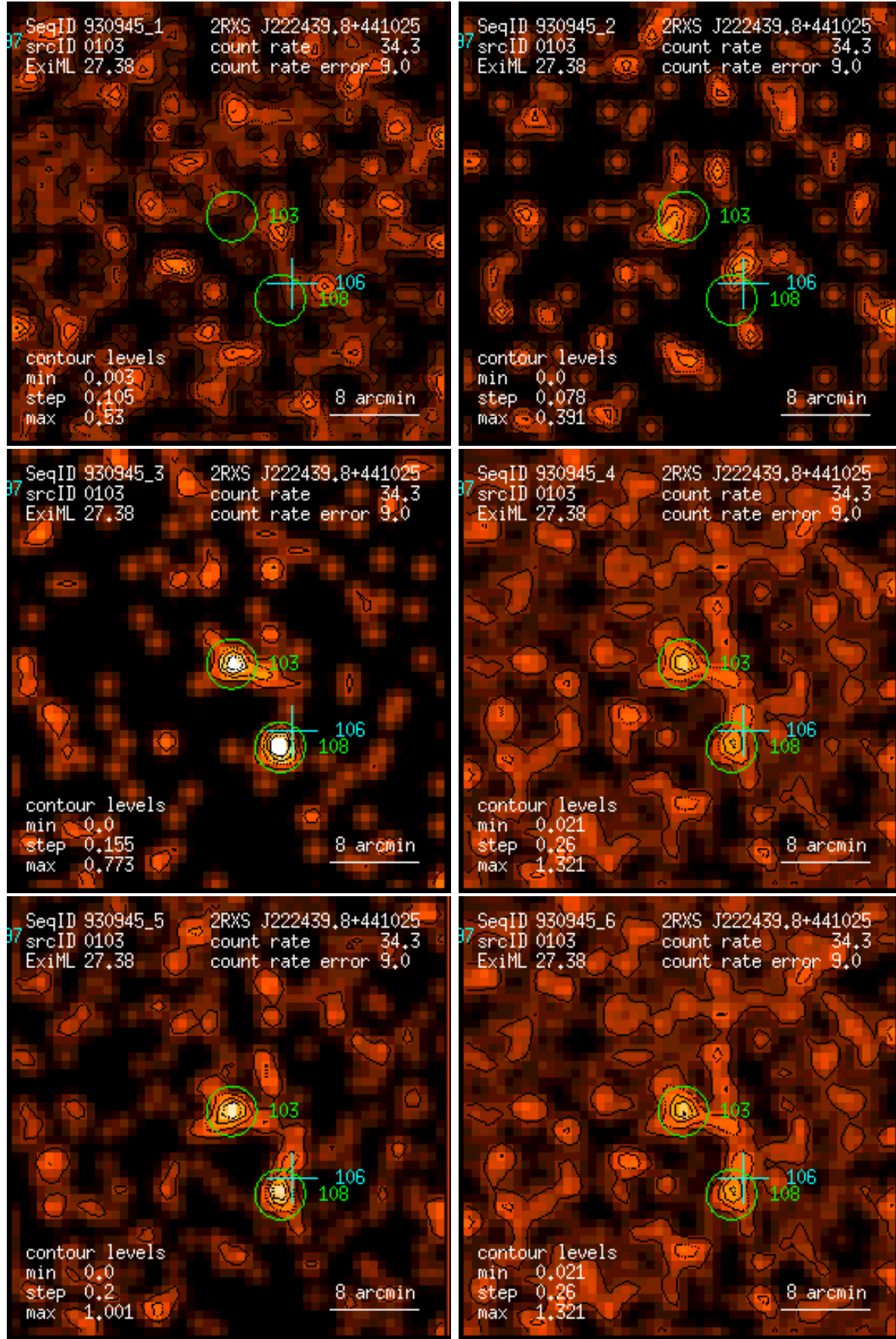
Figure 103: RASS 930945: detection 0103: band rate images, Gaussian filter: (1) PSPC channels 11 – 41, (2) 52 – 90, (3) 91 – 201, (4) 11 – 235, (5) 52 – 201, (6) 11 – 201. Broad band rates in counts/ks. Band rate contour levels in counts/ks/arcmin 2 .
