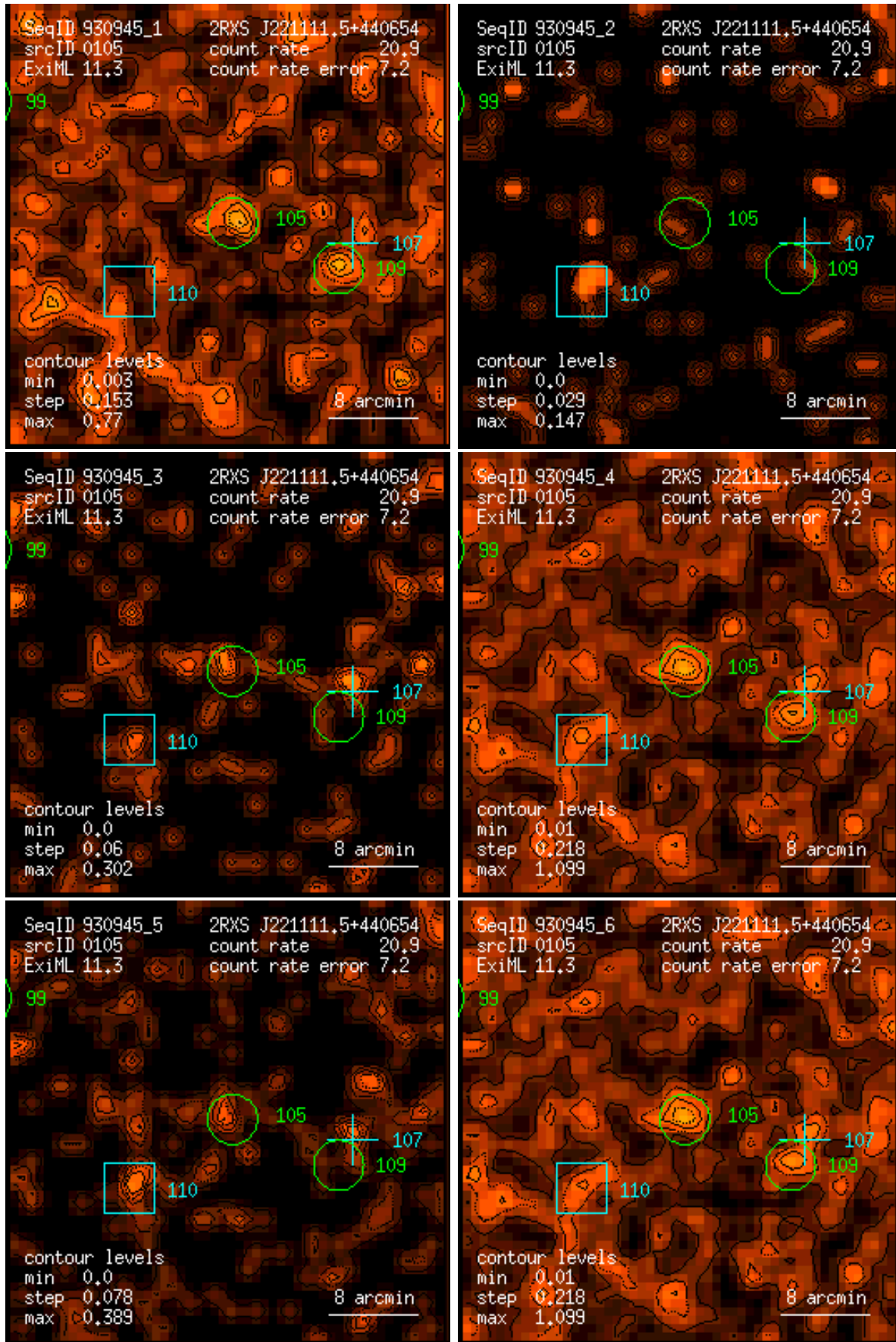
Figure 105: RASS 930945: detection 0105: band rate images, Gaussian filter: (1) PSPC channels 11 – 41, (2) 52 – 90, (3) 91 – 201, (4) 11 – 235, (5) 52 – 201, (6) 11 – 201. Broad band rates in counts/ks. Band rate contour levels in counts/ks/arcmin 2 .
