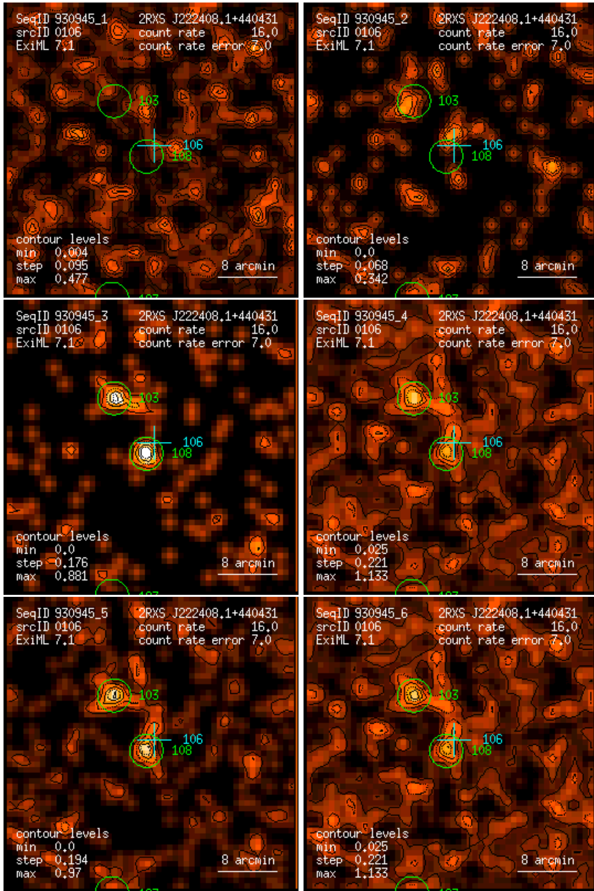
Figure 106: RASS 930945: detection 0106: band rate images, Gaussian filter: (1) PSPC channels 11 – 41, (2) 52 – 90, (3) 91 – 201, (4) 11 – 235, (5) 52 – 201, (6) 11 – 201. Broad band rates in counts/ks. Band rate contour levels in counts/ks/arcmin 2 .
