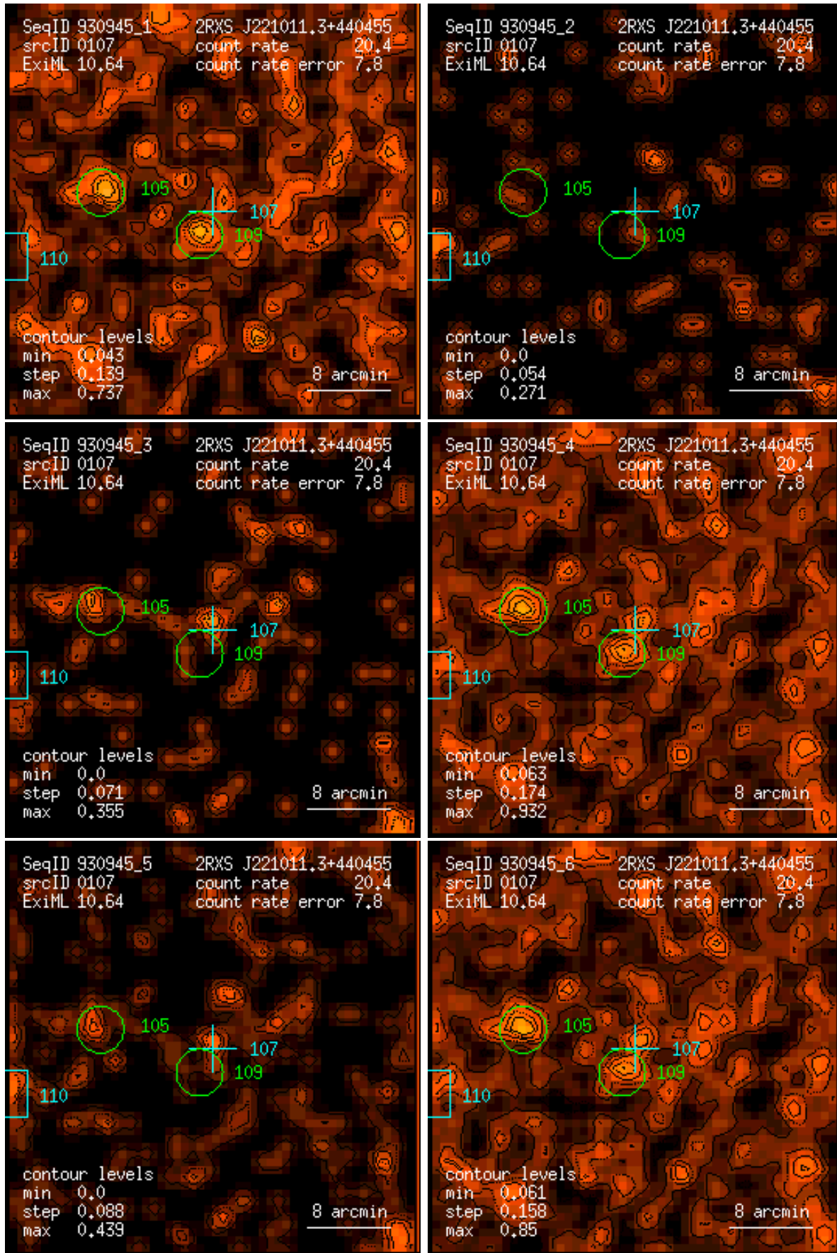
Figure 107: RASS 930945: detection 0107: band rate images, Gaussian filter: (1) PSPC channels 11 – 41, (2) 52 – 90, (3) 91 – 201, (4) 11 – 235, (5) 52 – 201, (6) 11 – 201. Broad band rates in counts/ks. Band rate contour levels in counts/ks/arcmin 2 .
