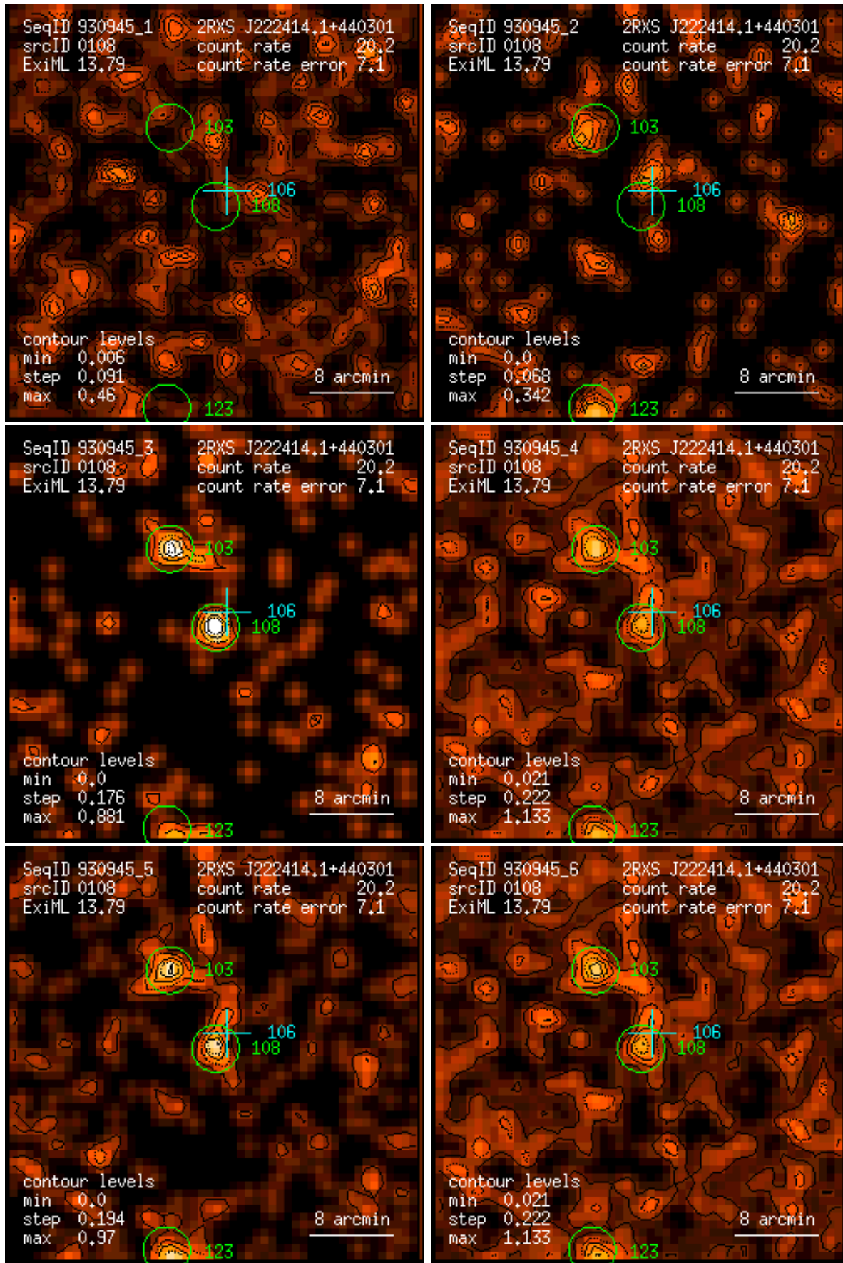
Figure 108: RASS 930945: detection 0108: band rate images, Gaussian filter: (1) PSPC channels 11 – 41, (2) 52 – 90, (3) 91 – 201, (4) 11 – 235, (5) 52 – 201, (6) 11 – 201. Broad band rates in counts/ks. Band rate contour levels in counts/ks/arcmin 2 .
