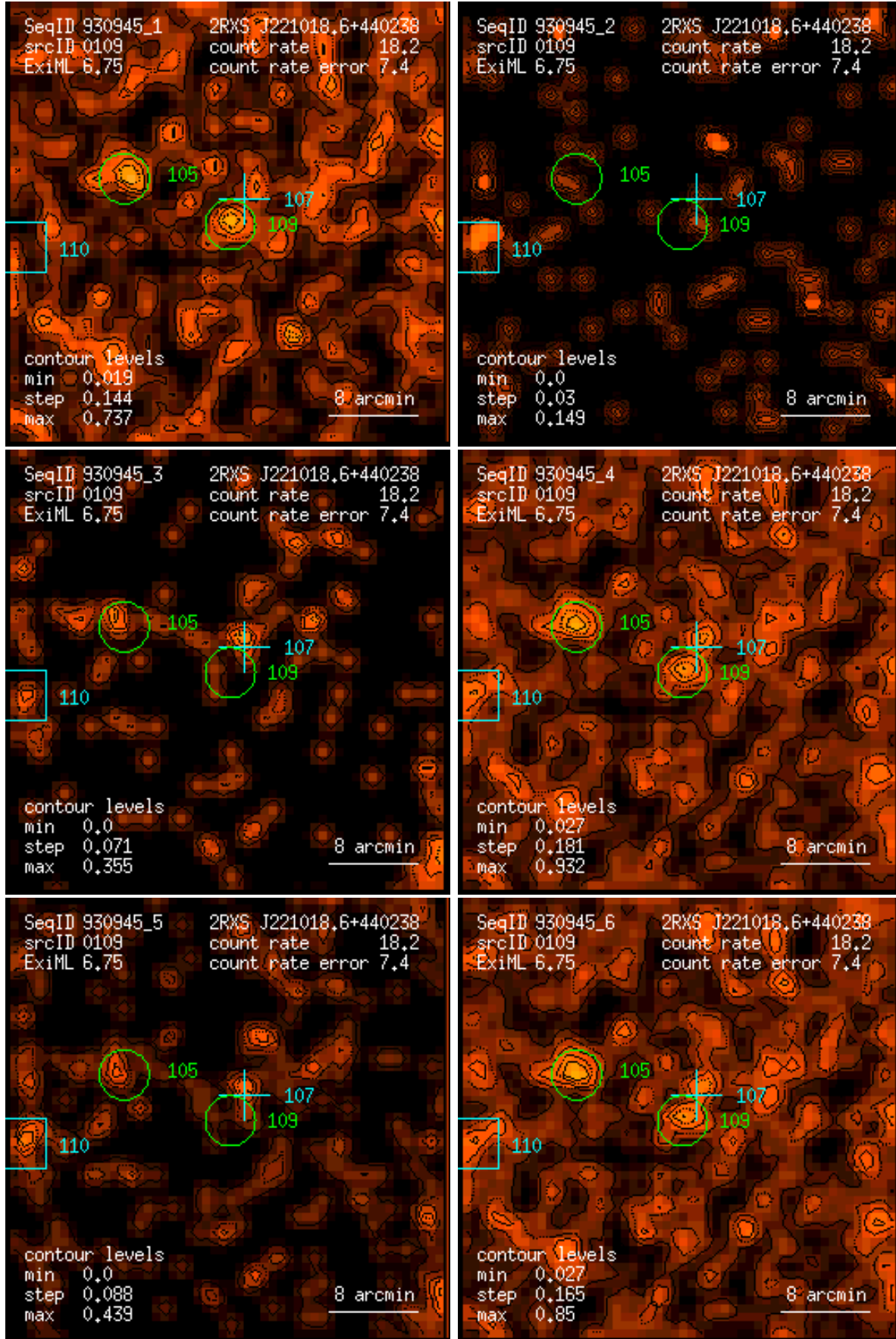
Figure 109: RASS 930945: detection 0109: band rate images, Gaussian filter: (1) PSPC channels 11 – 41, (2) 52 – 90, (3) 91 – 201, (4) 11 – 235, (5) 52 – 201, (6) 11 – 201. Broad band rates in counts/ks. Band rate contour levels in counts/ks/arcmin 2 .
